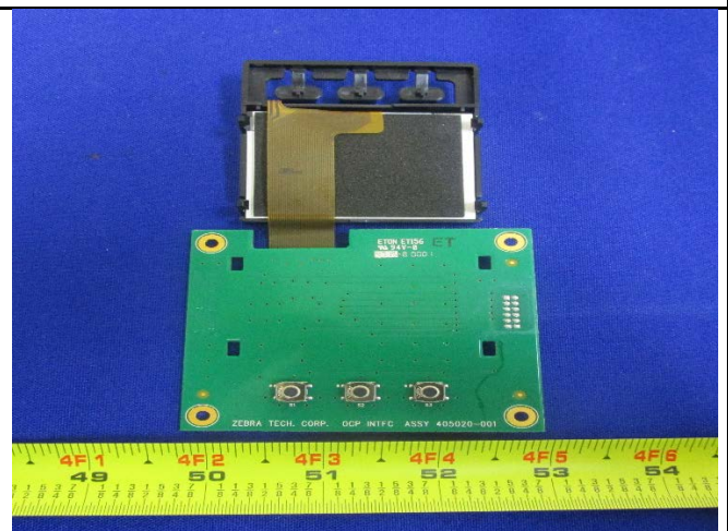
Display Board Bottom View 2
