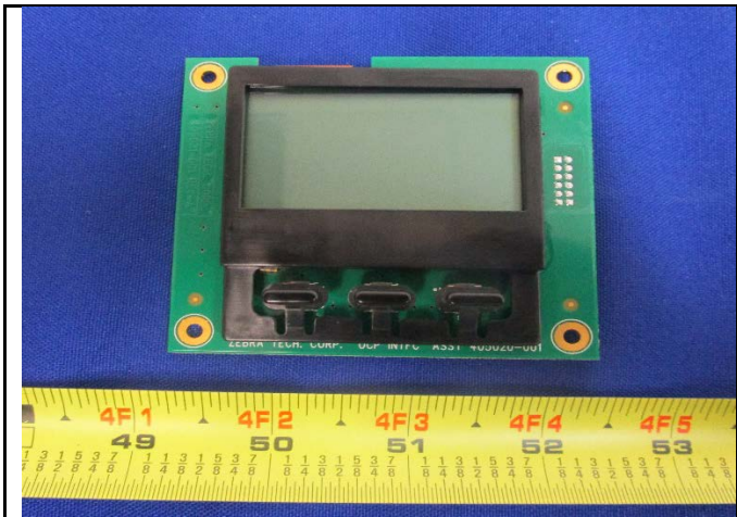
Display Board Top View 1
