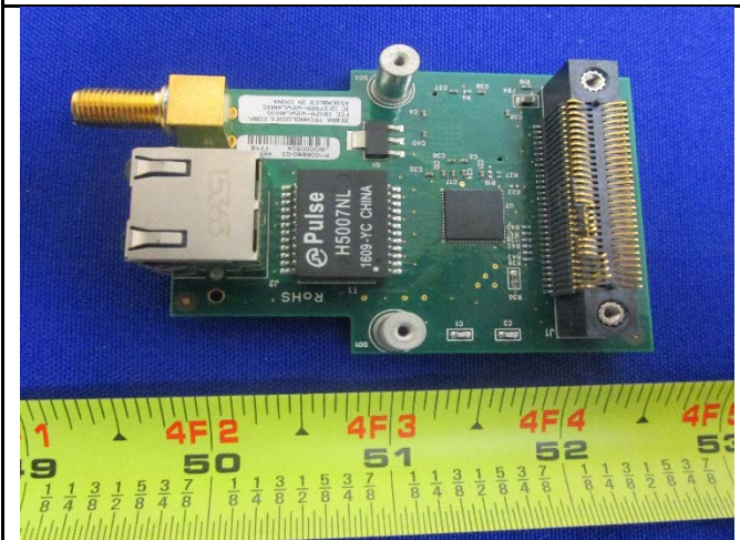
WIFI Radio Board Top View
