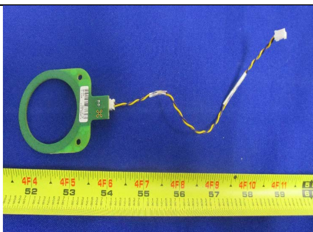
Ribbon RFID2 Antenna Bottom View
