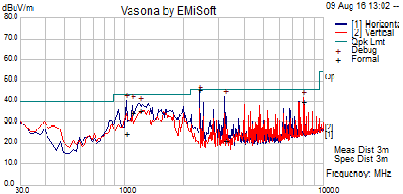
f=30MHz – 1000MHz plot and 3 meter distance
