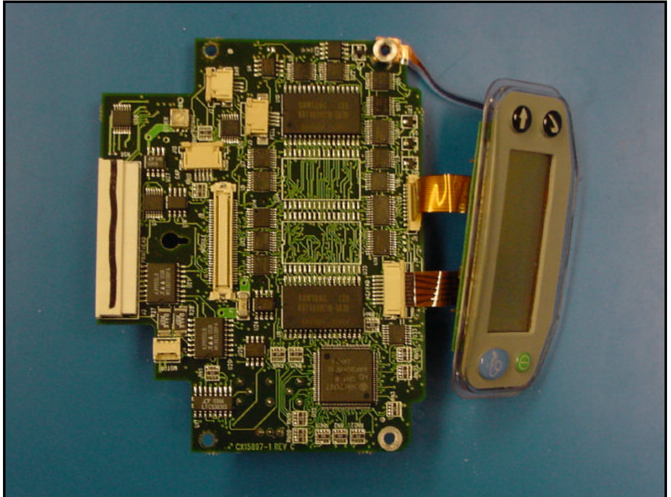
PHOTOGRAPH 18: PCB1 TOP WITH LCD DISPLAY
