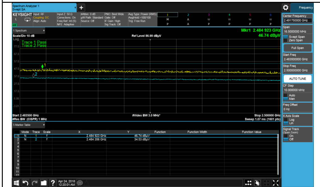
802.11n-HT40-2452MHz
