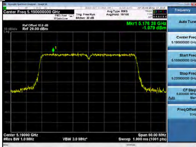
PSD-802.11n-40M 5190MHz
