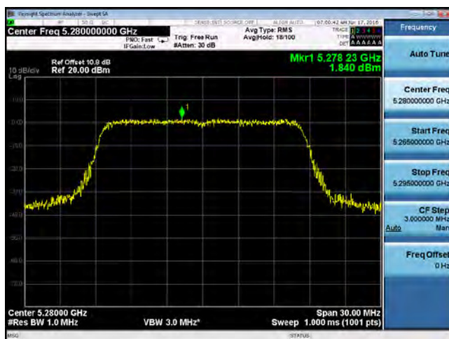
PSD-802.11a 5280MHz
