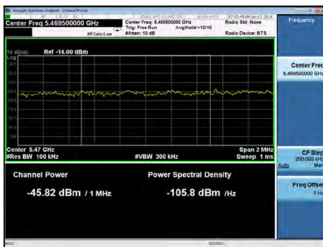
Band Edge-802.11a 5500 MHz (Limit: -27dBm/MHz eirp)
