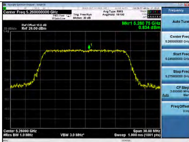
PSD-802.11a 5260MHz
