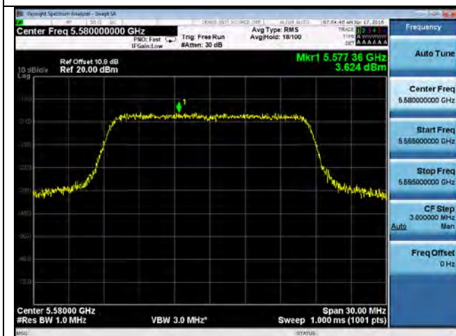
PSD-802.11a 5580MHz
