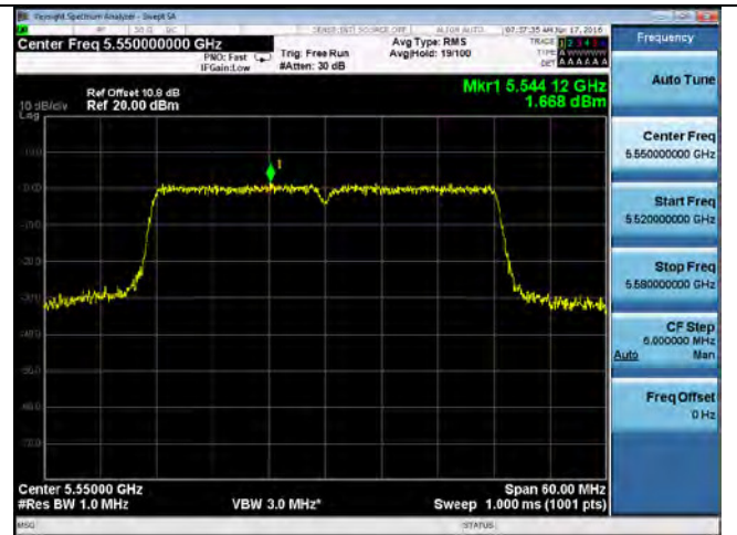
PSD-802.11n-40M 5550MHz
