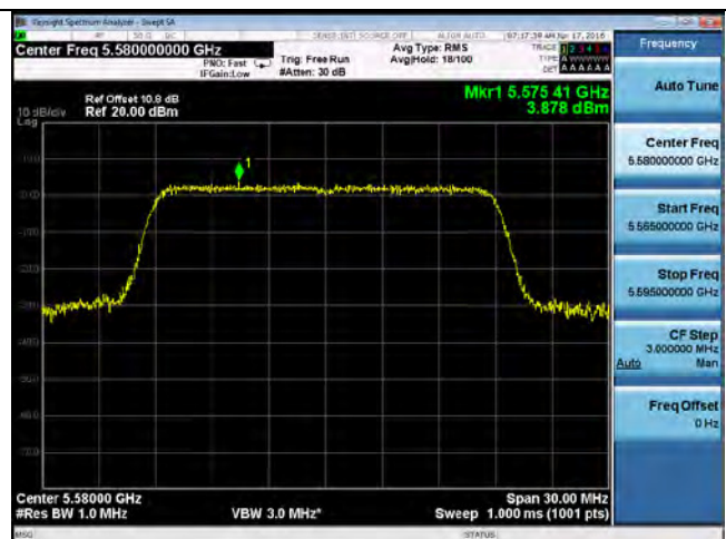
PSD-802.11n-20M 5580MHz
