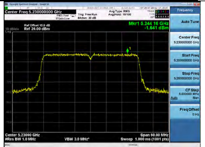
PSD-802.11n-40M 5230MHz
