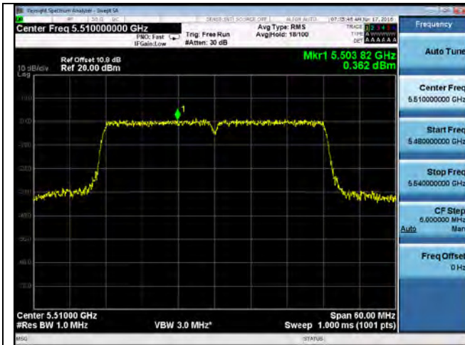
PSD-802.11n-40M 5510MHz
