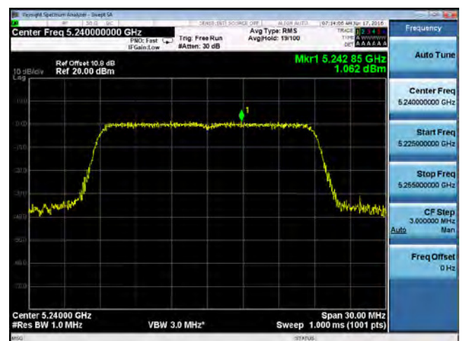
PSD-802.11n-20M 5240MHz
