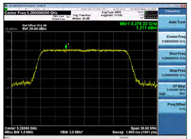
PSD-802.11n20M 5280MHz
