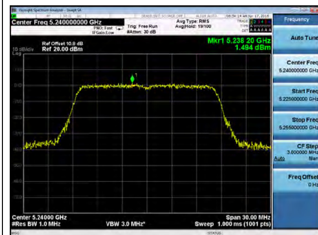
PSD-802.11a 5240MHz
