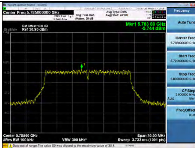
PSD-802.11a 5785MHz
