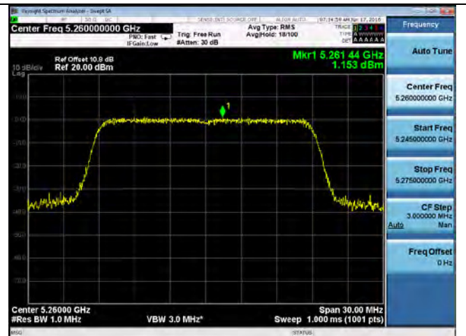
PSD-802.11n-20M 5260MHz
