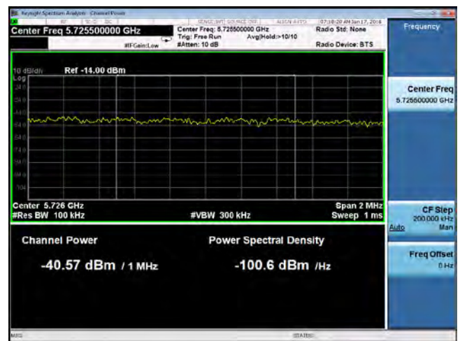
Band Edge-802.11n20 5700 MHz (Limit: -27dBm/MHz eirp)
