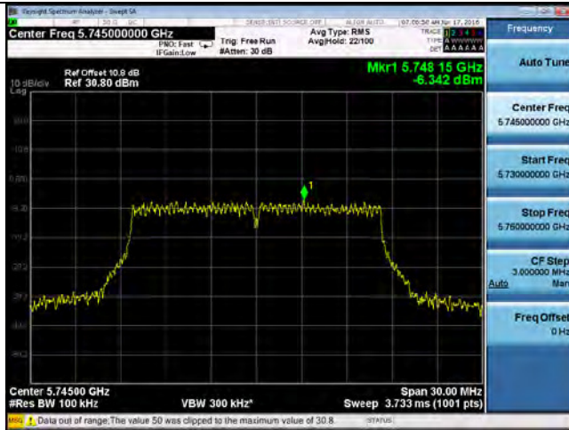
PSD-802.11a 5745MHz
