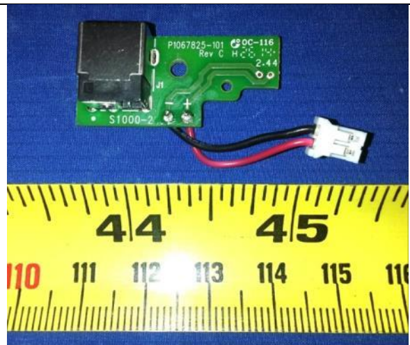
Power Board Top View
