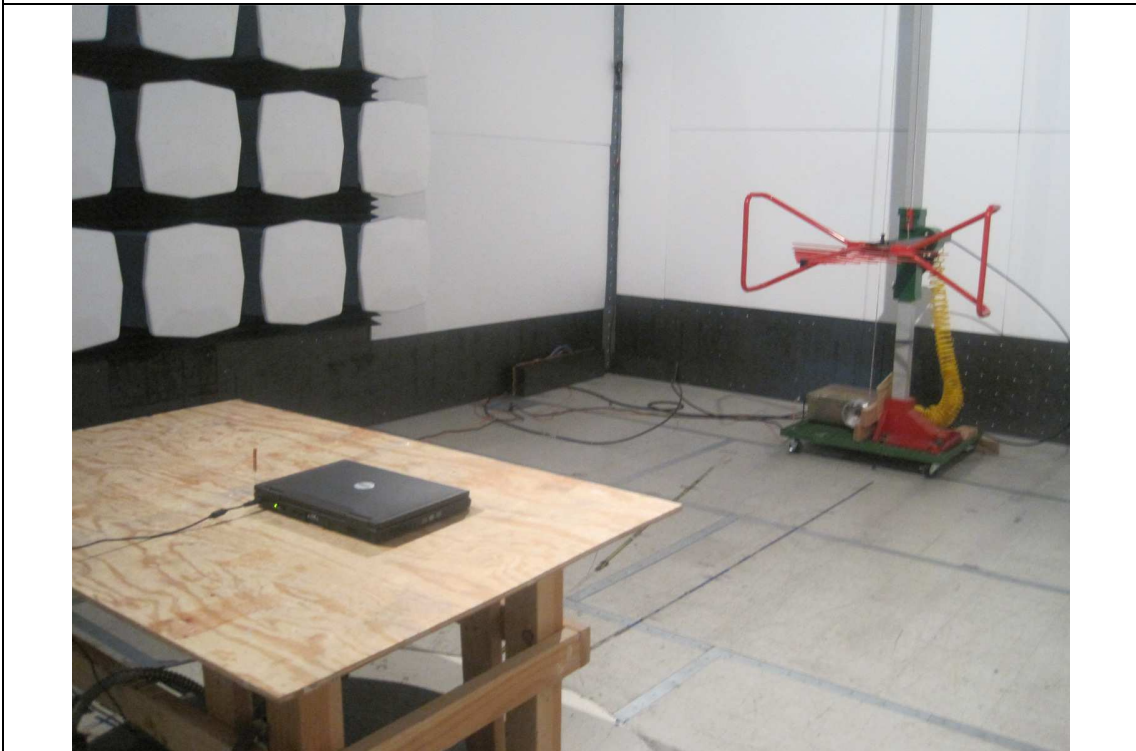
Radiated Emission Test Setup with patch antenna (30MHz – 1GHz) – Rear View
