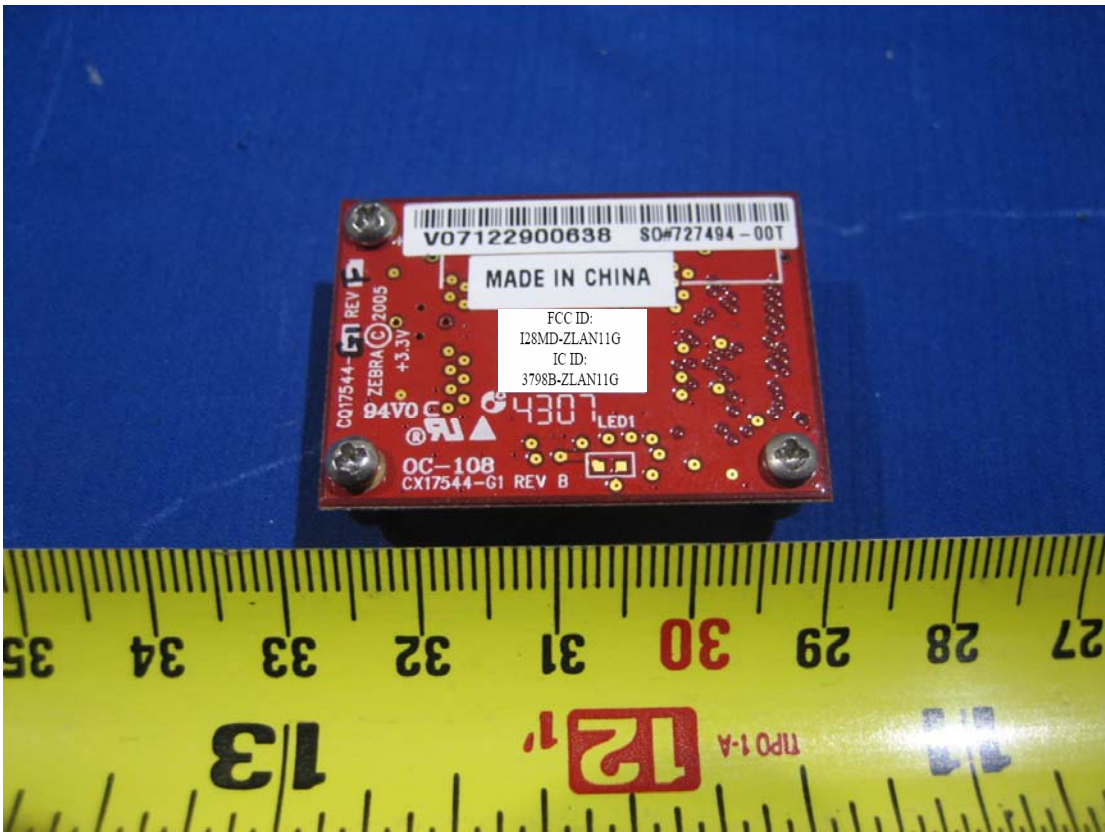
Radio Module Solder View
