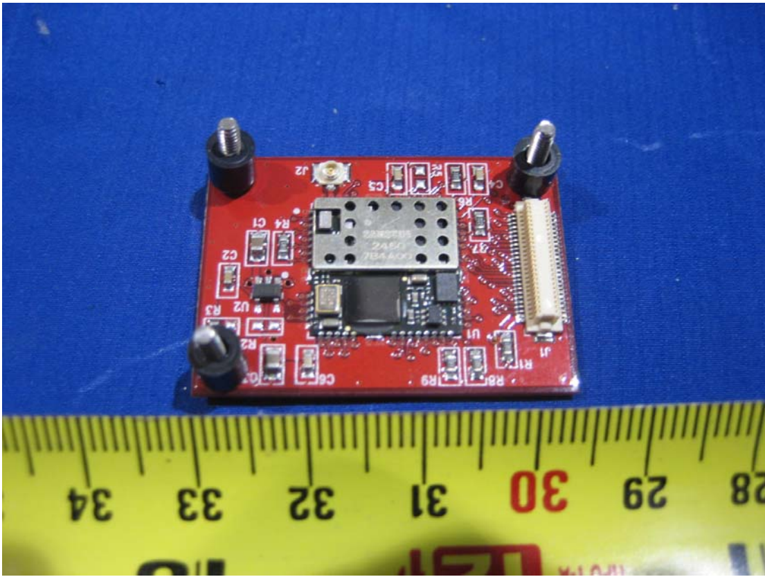
Radio Module Component View
