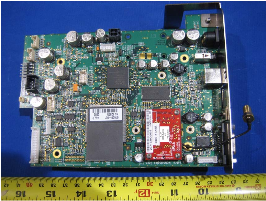
Main Board Component View
