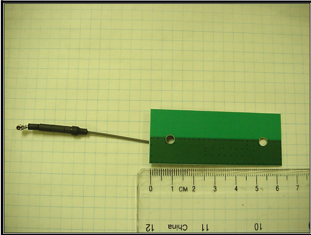
Photograph 14: CQ17810-G3M (QL420+) - PICA; Back View
