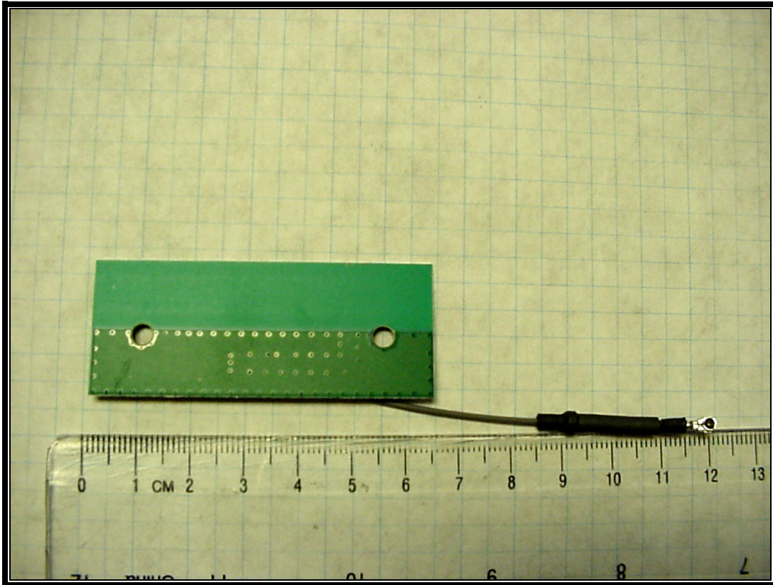
Photograph 12: CQ17810-G2M (QL320+) - PICA; Back View
