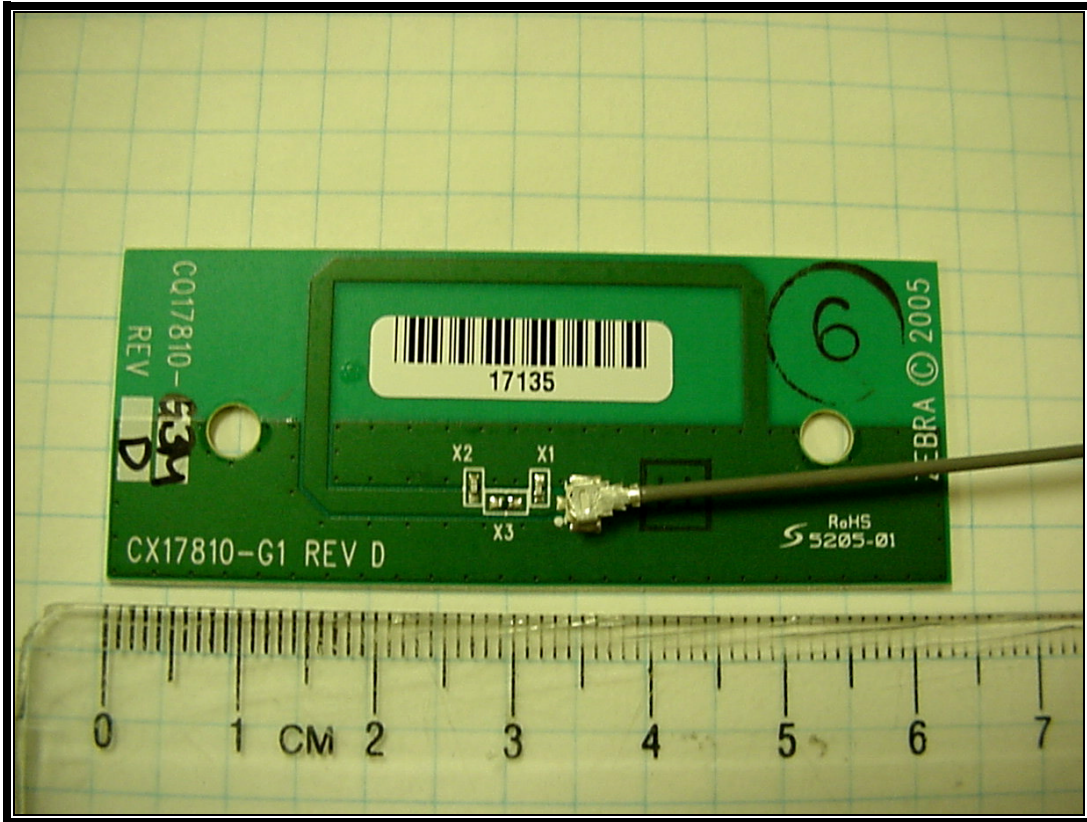
Photograph 13: CQ17810-G3M (QL420+) - PICA; Front View
