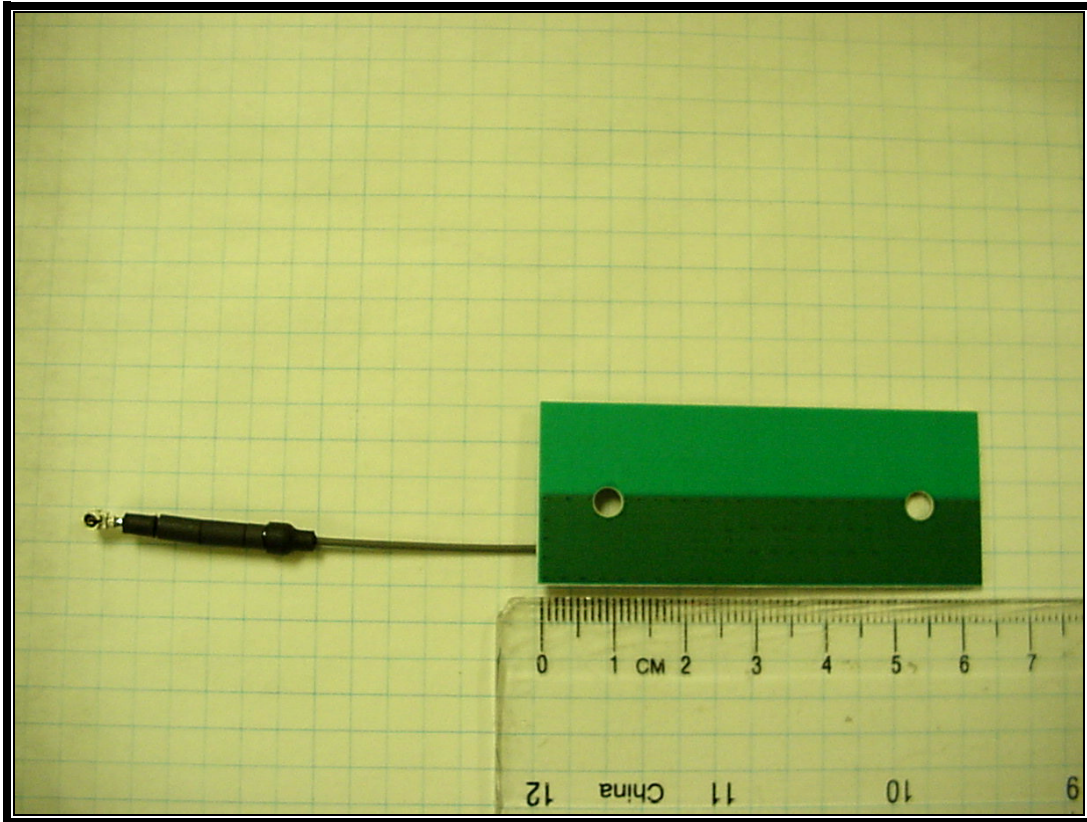
Photograph 10: CQ17810-G1M (QL220+) - PICA; Back View
