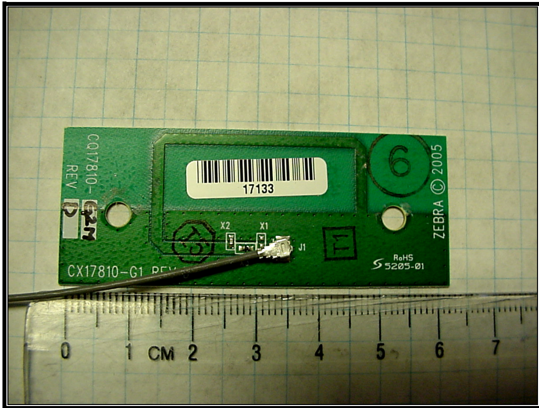
Photograph 11: CQ17810-G2M (QL320+) - PICA; Front View
