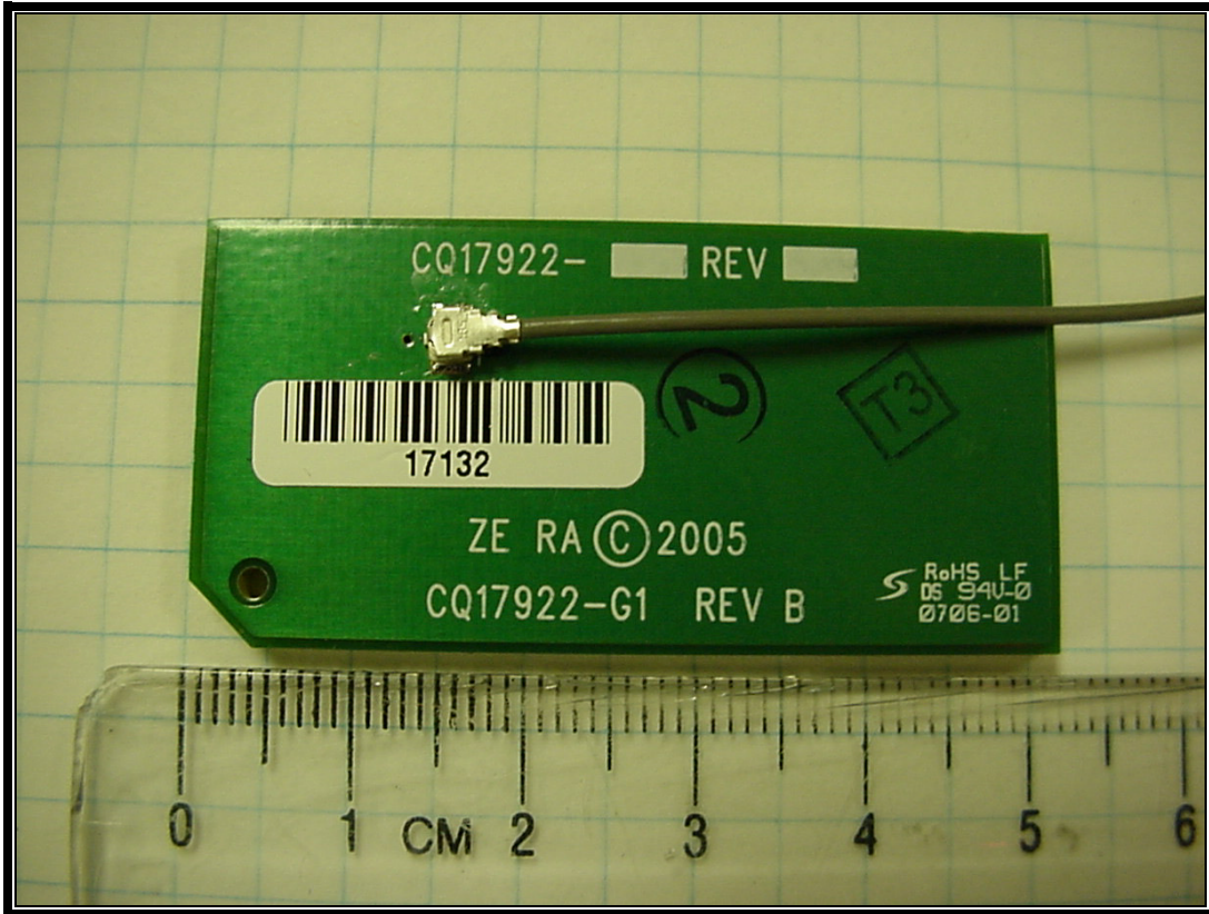
Photograph 7: CQ17922-G1 (GENIII print server) - Patch; Front View
