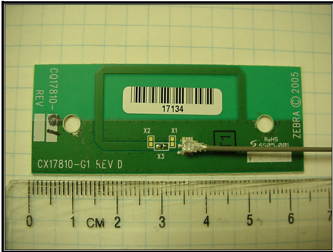
Photograph 9: CQ17810-G1M (QL220+) - PICA; Front View
