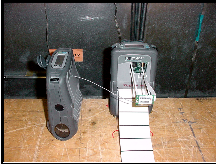
CONDUCTED EMISSIONS FRONT VIEW USING QL-420 CQ17383-1
