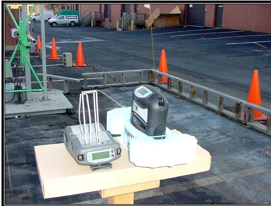
PHOTOGRAPH 7: RADIATED EMISSIONS FRONT VIEW USING RW-420 CQ17252-1 ANTENNA
