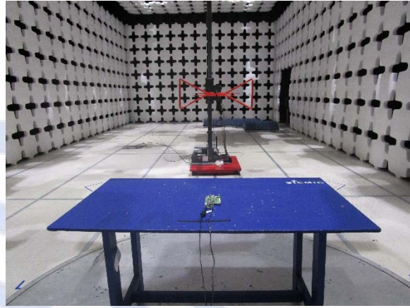
Radiated Emission Test setup (<1GHz) – Rear View
