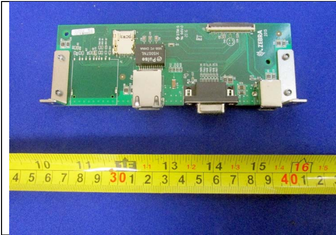
EUT PCBA I/O Board – Top View
