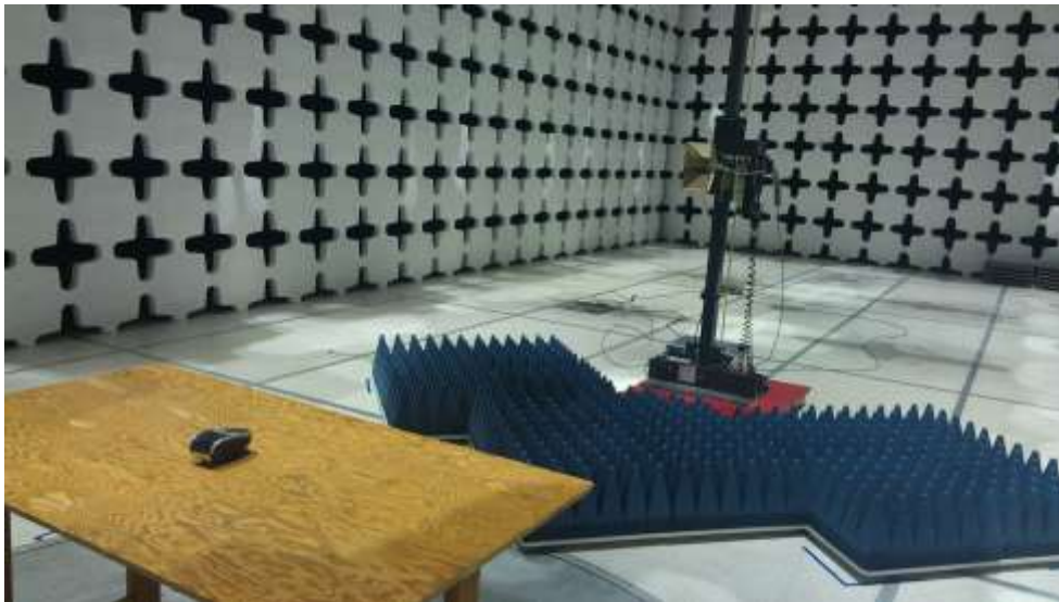
Radiated emissions above 1 GHz setup (iMZ220) - Back view
