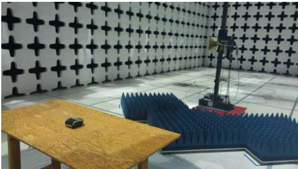
Radiated emissions above 1 GHz setup (iMZ320) - Back view
