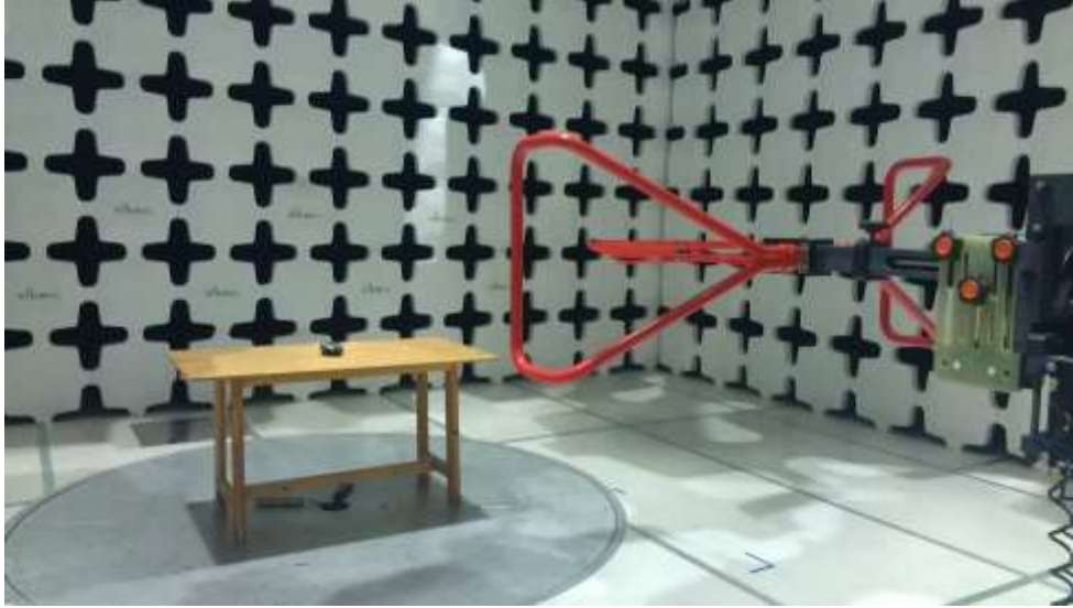
Radiated emissions below than 1 GHz setup (iMZ320) - Front view
