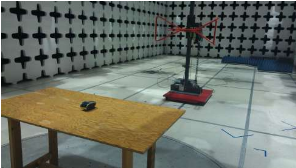
Radiated emissions below than 1 GHz setup (iMZ220) - Back view
