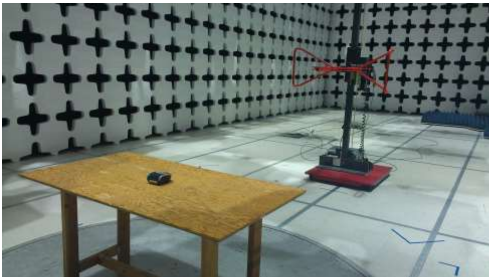
Radiated emissions below than 1 GHz setup (iMZ320) - Back view
