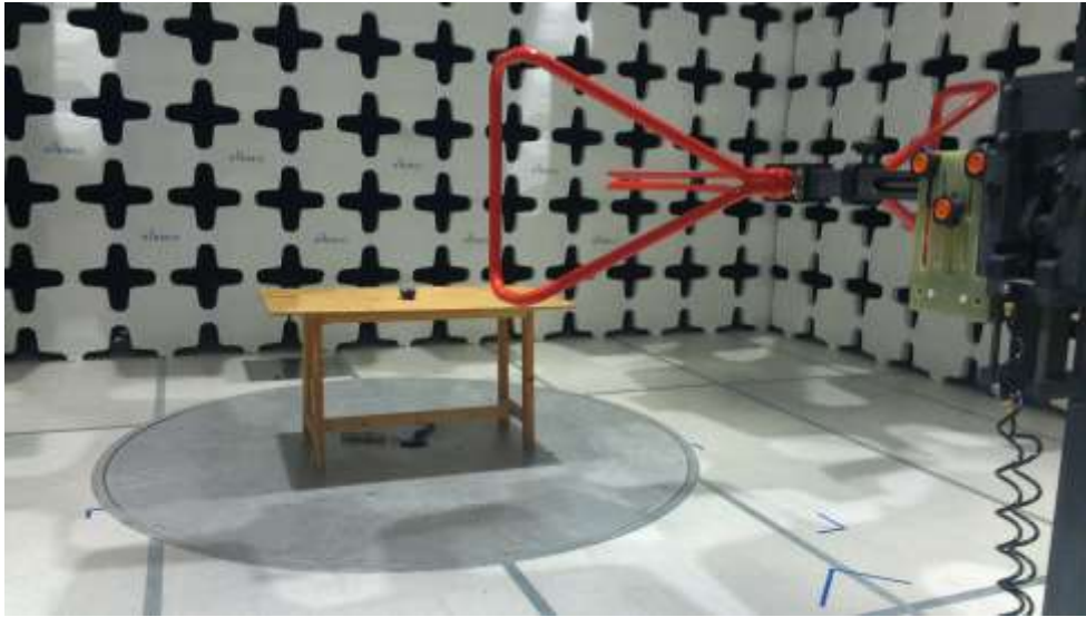
Radiated emissions below than 1 GHz setup (iMZ220) - Front view
