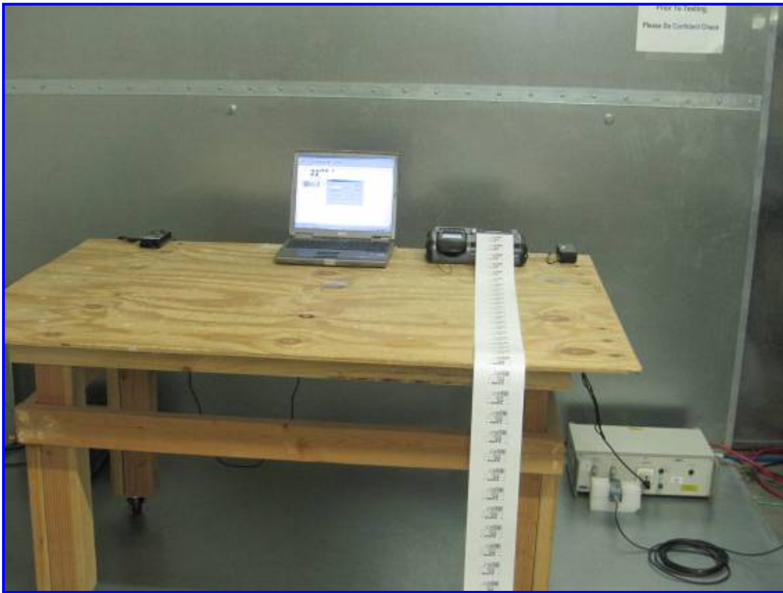
Conducted Emission Test Setup – Front View
