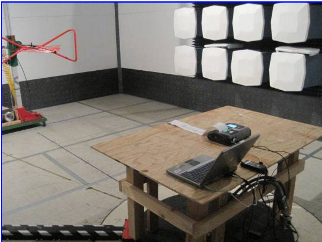
Radiated Emission Test Setup – Rear View
