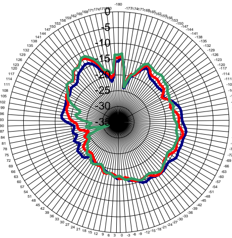
YZ plane - CQ17715-G1 RW220-BT antenna gain pattern
