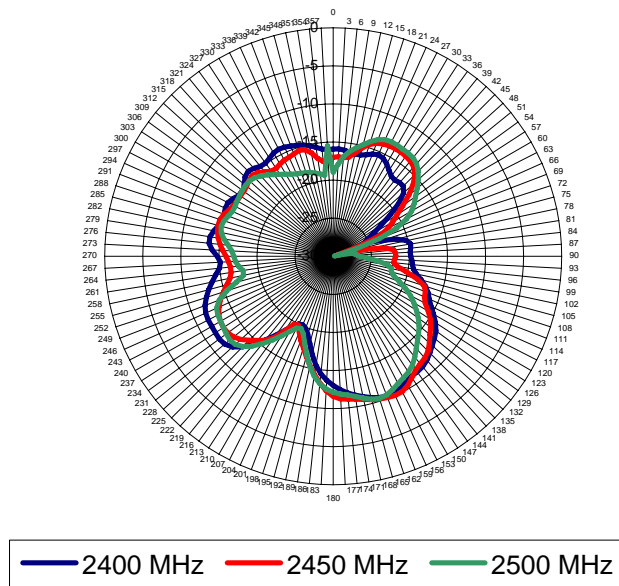
XY Plane - CQ17715-G1 RW220-BT antenna gain pattern
