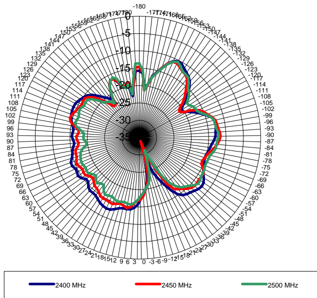
XZ plane - CQ17715-G1 RW220-BT antenna gain pattern
