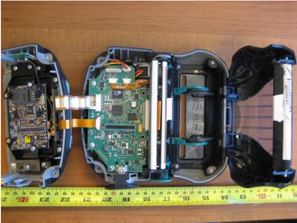
Host RW220 Cover Off
