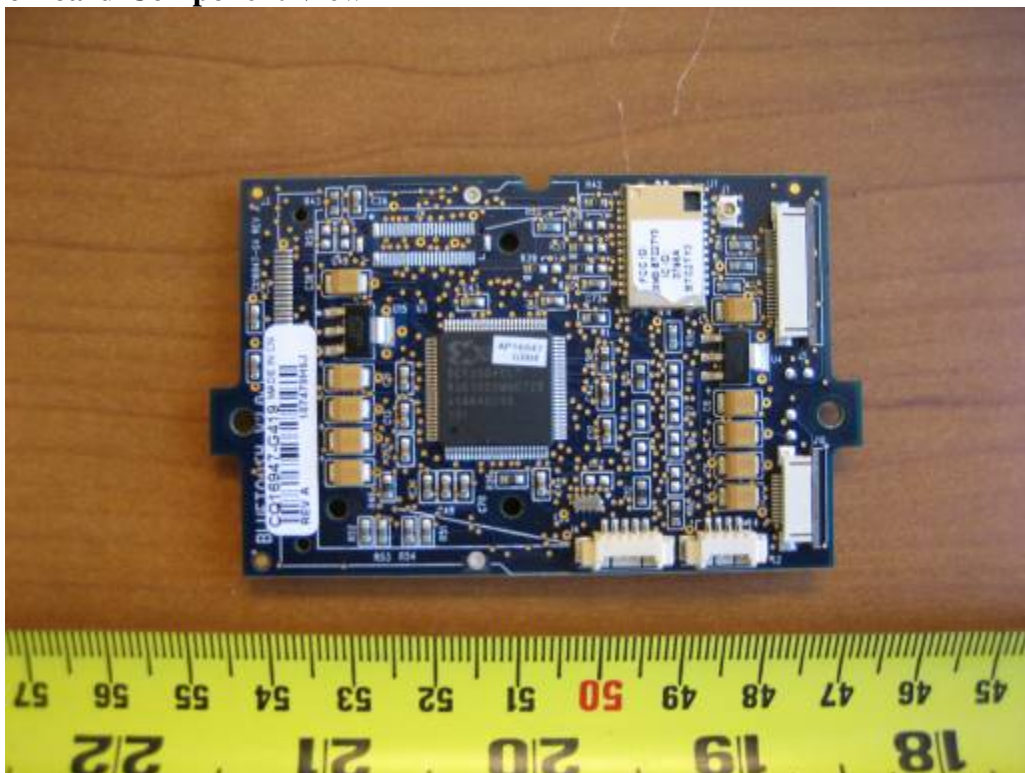
Radio Board-Component View 1
