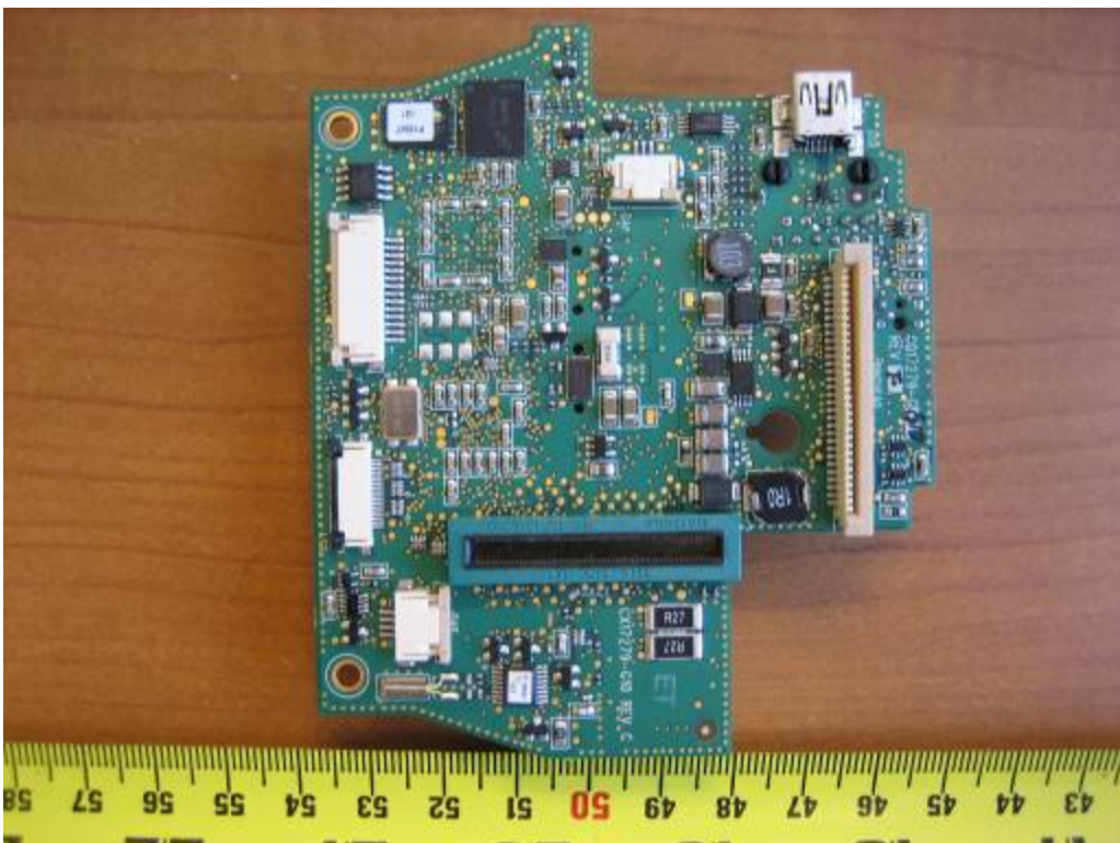
Main Board-component view-1
