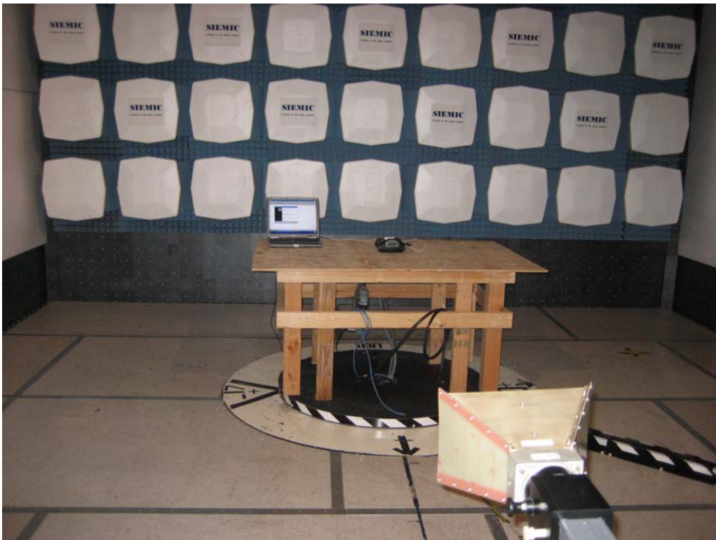
Above 1GHz Host EUT RW420
