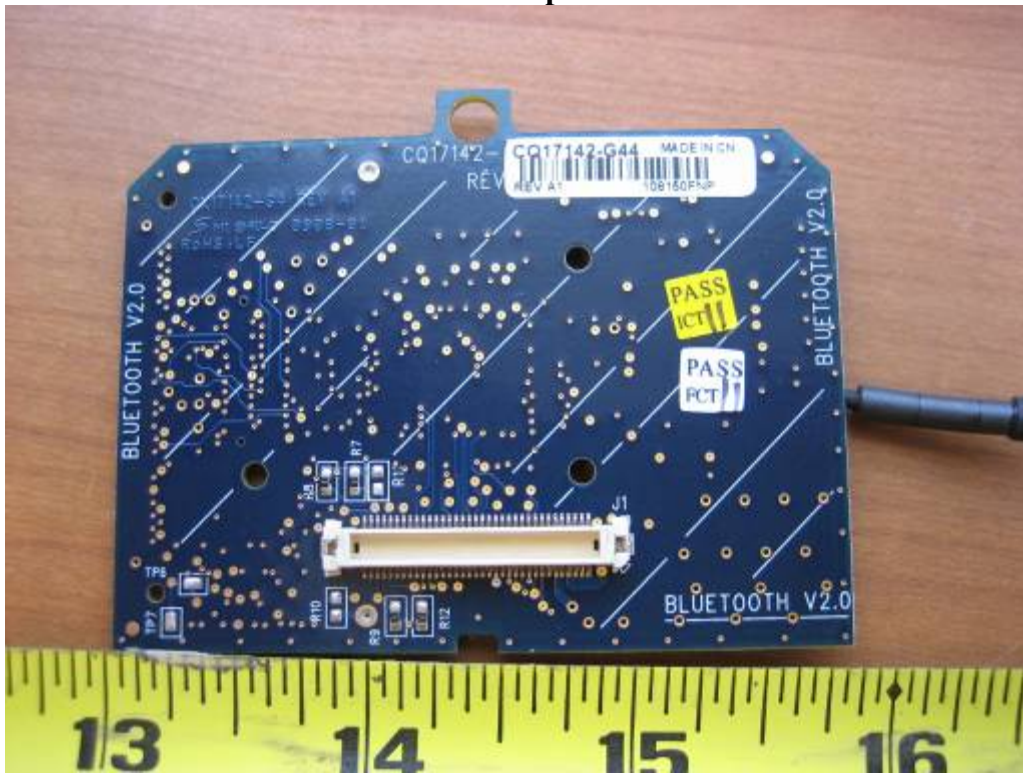
Antenna View -1
