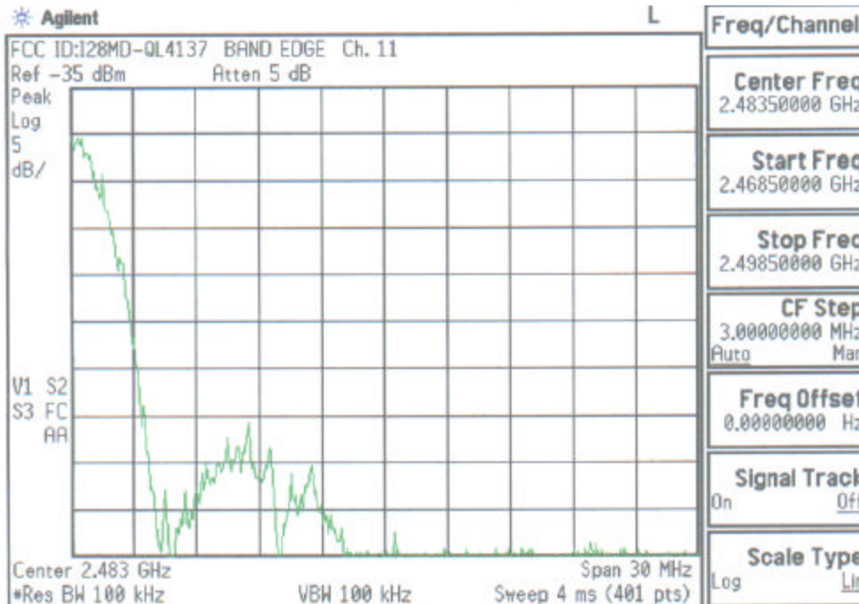
Plot A-12. BandEdge Plot – Ch.11
