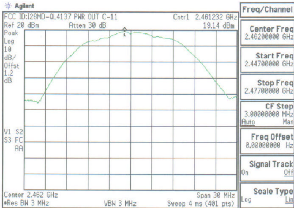
Plot A-6. Max. Peak Output Power Plot – Ch.11
