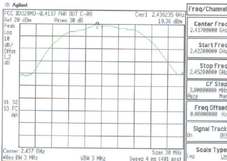
Plot A-5. Max. Peak Output Power Plot – Ch.6
