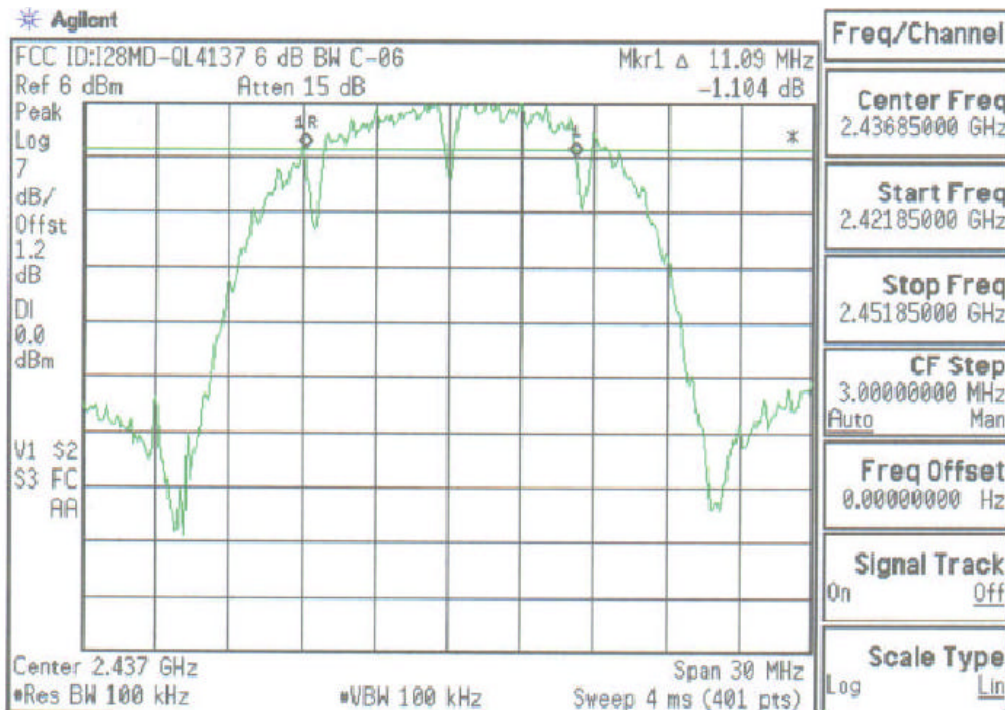
Plot A-2. 6dB Bandwidth Plot – Ch.6
