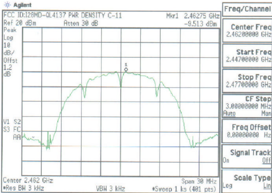
Plot A-9. Max. Power Density Plot – Ch.11
