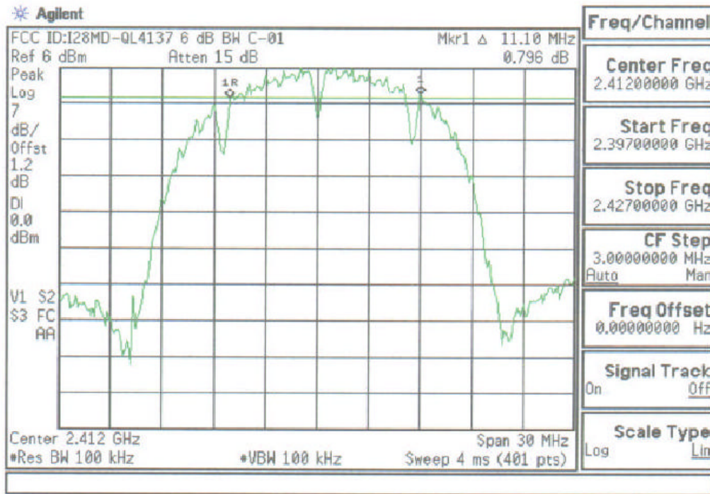
Plot A-1. 6dB Bandwidth Plot – Ch.1
