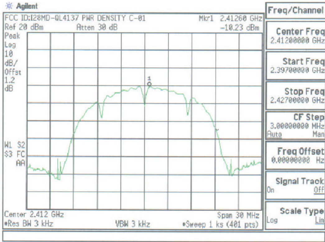
Plot A-7. Max. Power Density Plot – Ch.1
