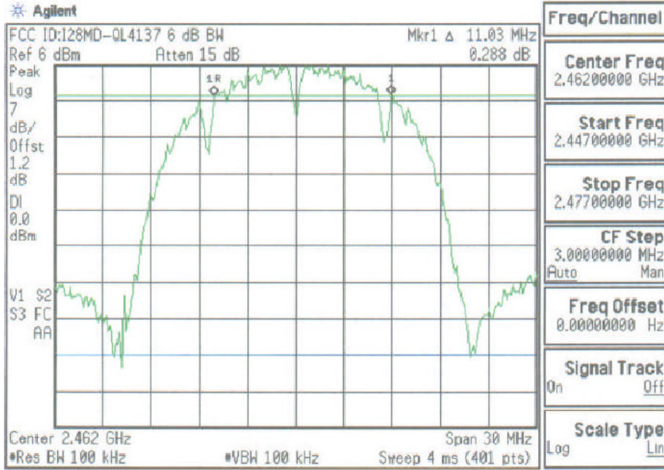
Plot A-3. 6dB Bandwidth Plot – Ch.11
