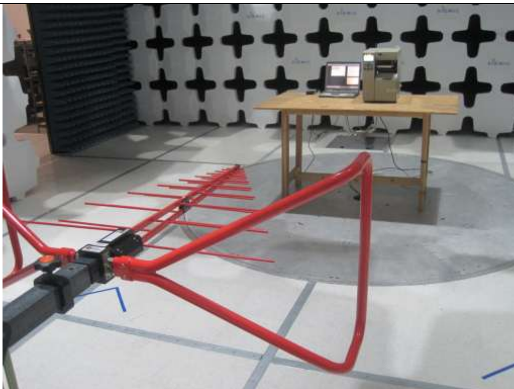
Radiated Emission Test (30MHz – 1GHz) - Front View
