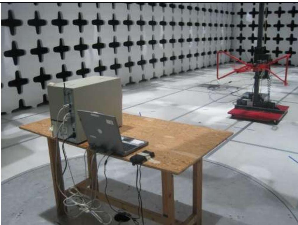
Radiated Emission Test Setup (30MHz – 1GHz) – Rear View
