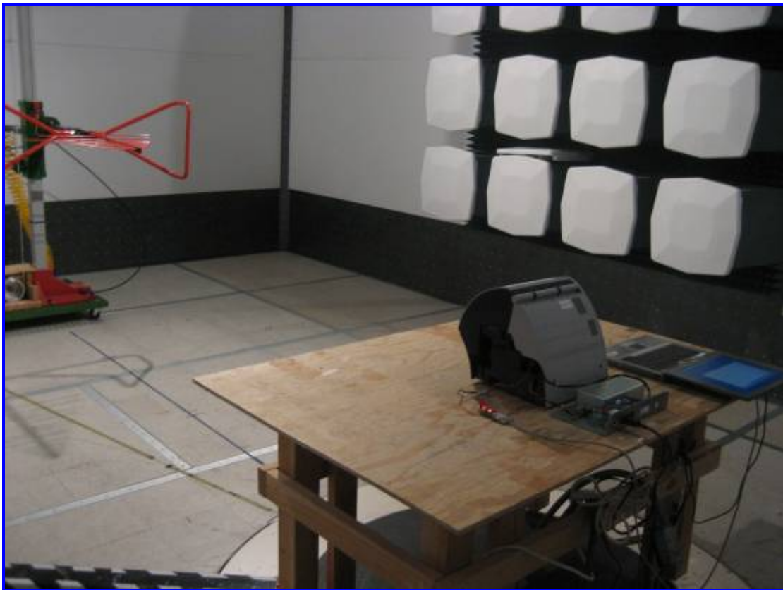
Radiated Emission Test Setup Rear View (<1000MHz)
