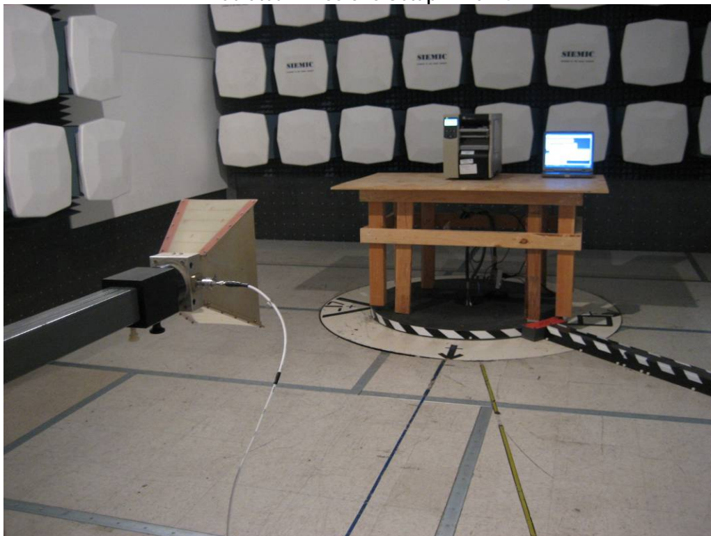
Radiated Emissions Setup - 220Xi4
