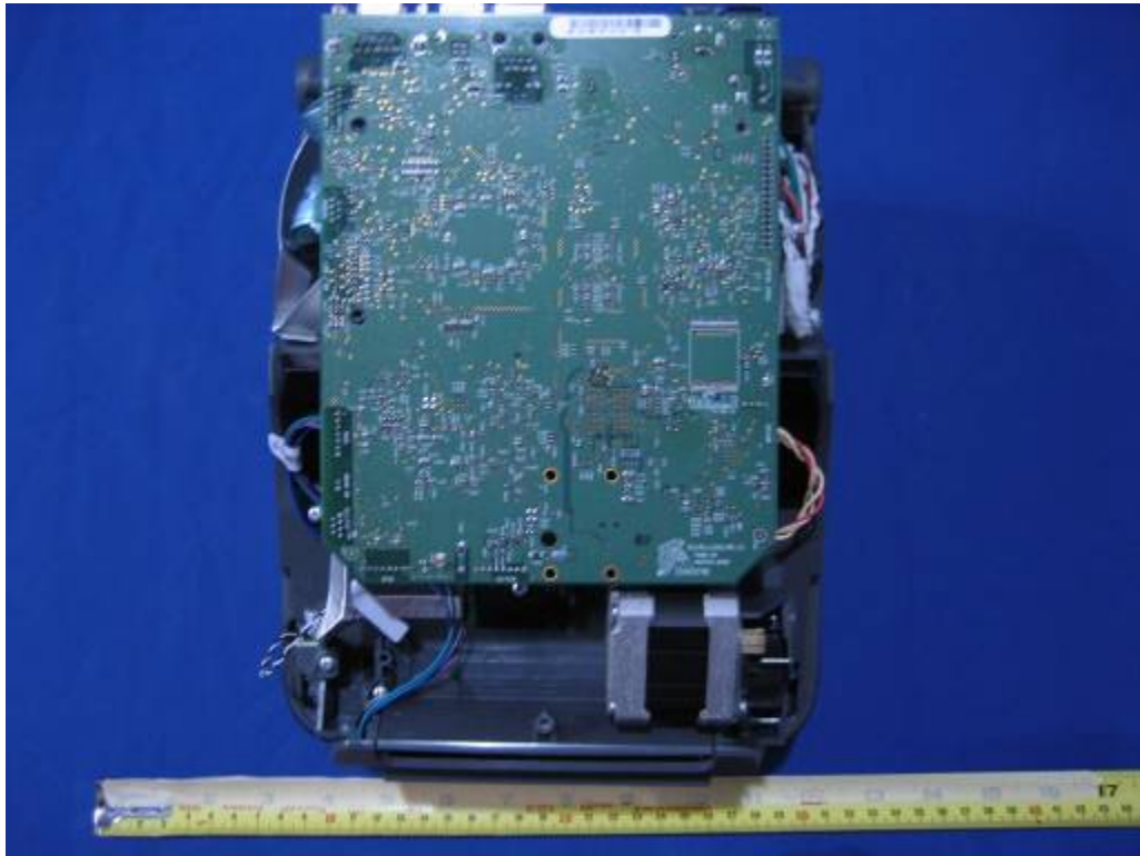
Cover Off -2
