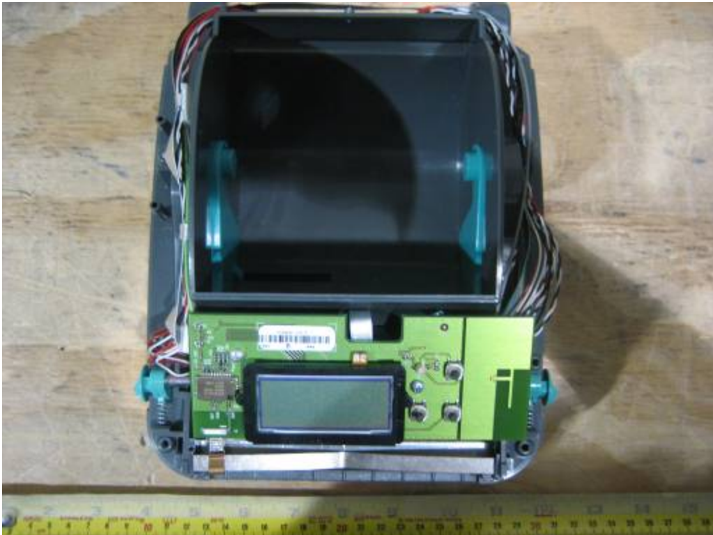
Cover Off -1
