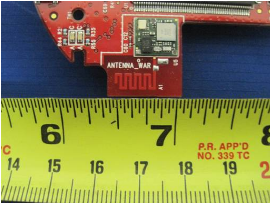
Radio Module without RF shield
