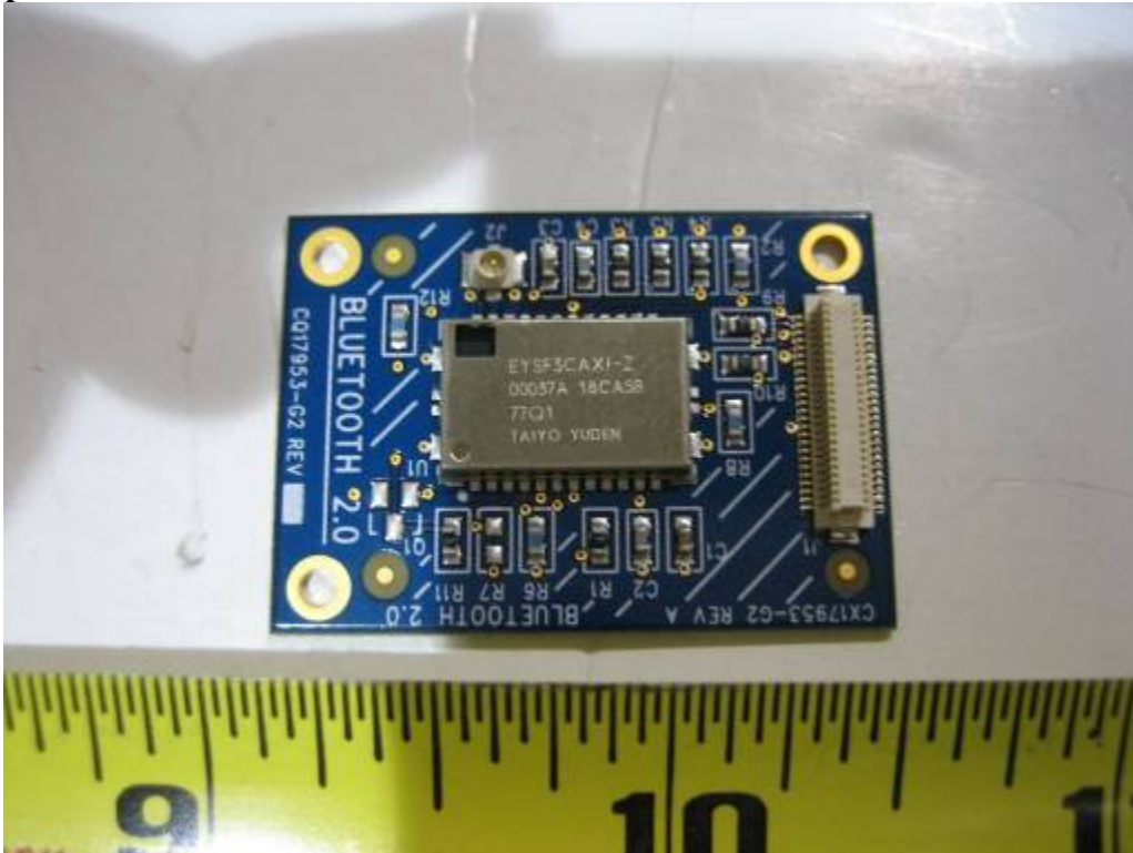
EUT Photo-Bluetooth Component View-1
