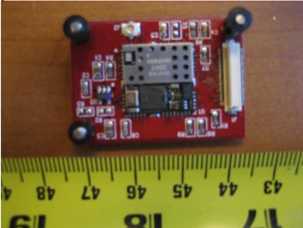
EUT Photo-WLAN Component View-1
