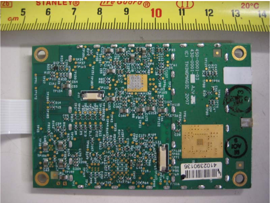
Solder View
