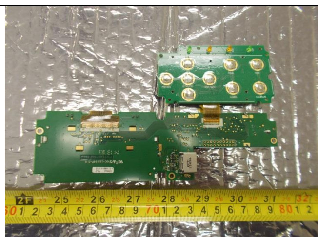
Sub LED PCBA 5 - Bottom View
