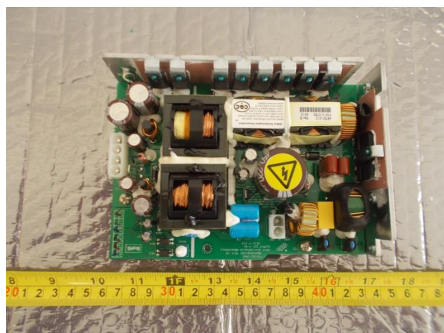
Internal Power Supply - Top View
