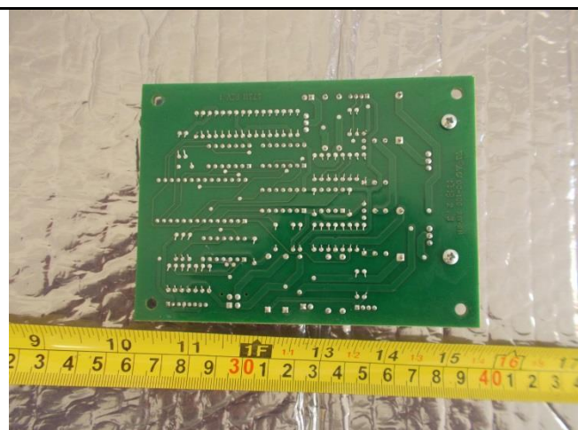
Sub PCBA 3 Bottom View
