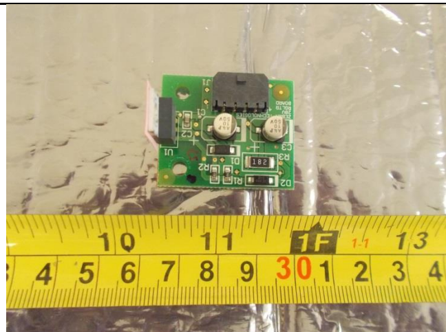
Sub PCBA 6 - Top View
