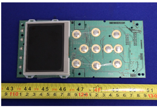
LCD board - Top view
