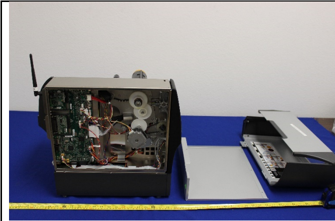
EUT - Cover off-1
