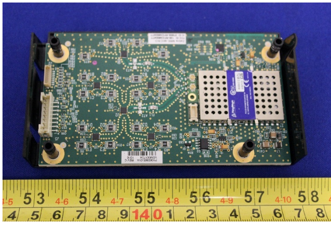
UHF RFID Board - Top view
