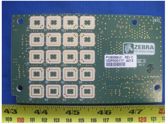
RFID Radio Module & Antenna – Bottom view
