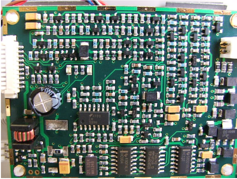
RFID board
