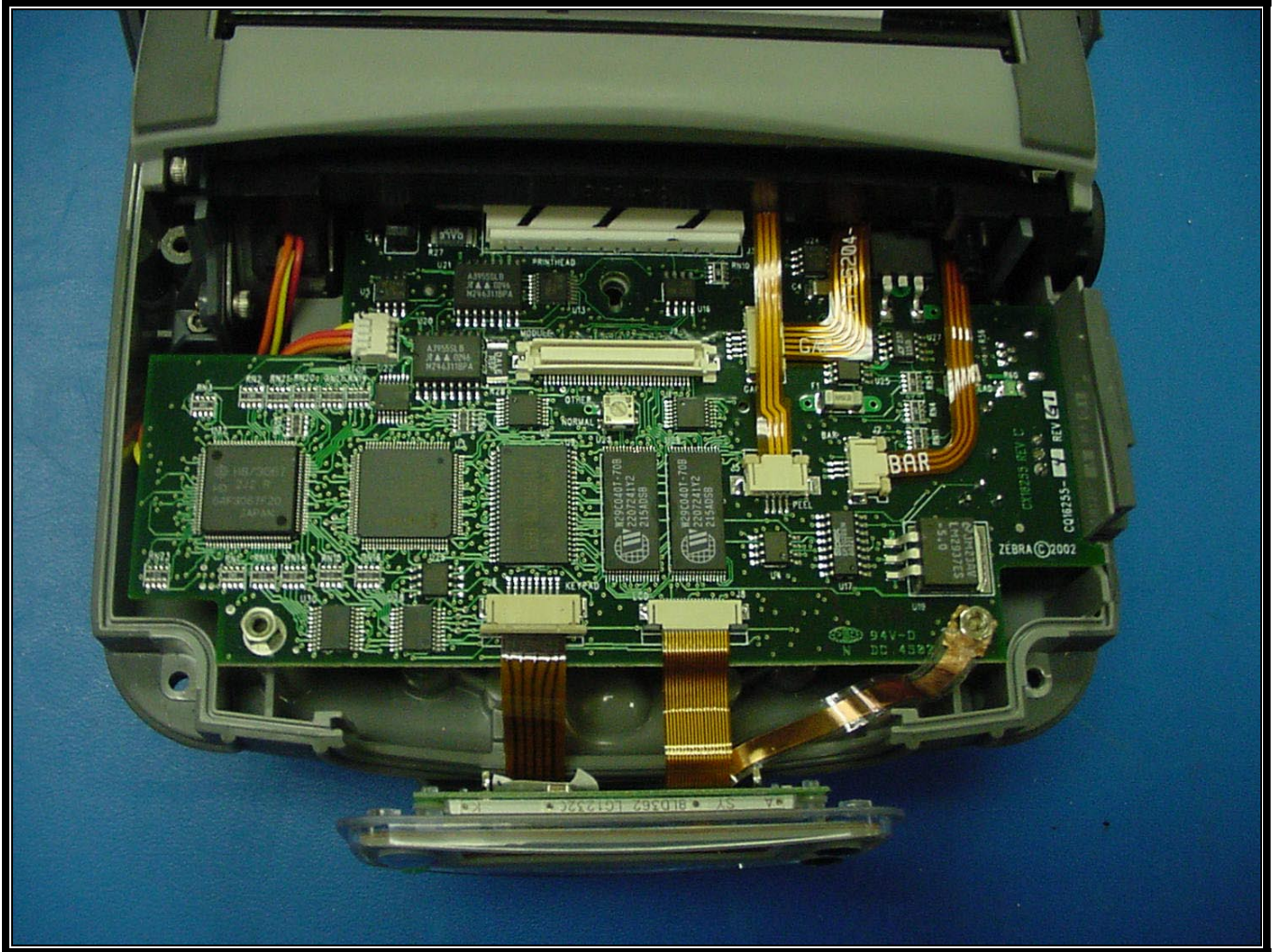
PHOTOGRAPH 12: INSIDE PCB
