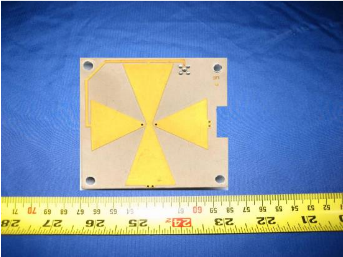
UHF Antenna Front View
