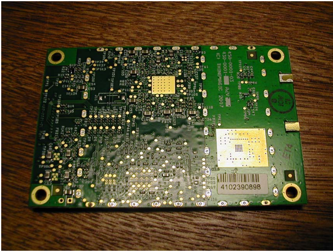
UHF Module Solder View
