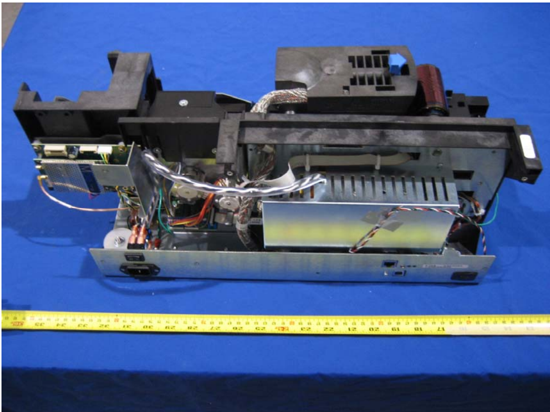
Cover off Rear View
