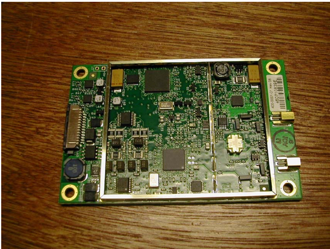
UHF Module Component View Shielding OFF
