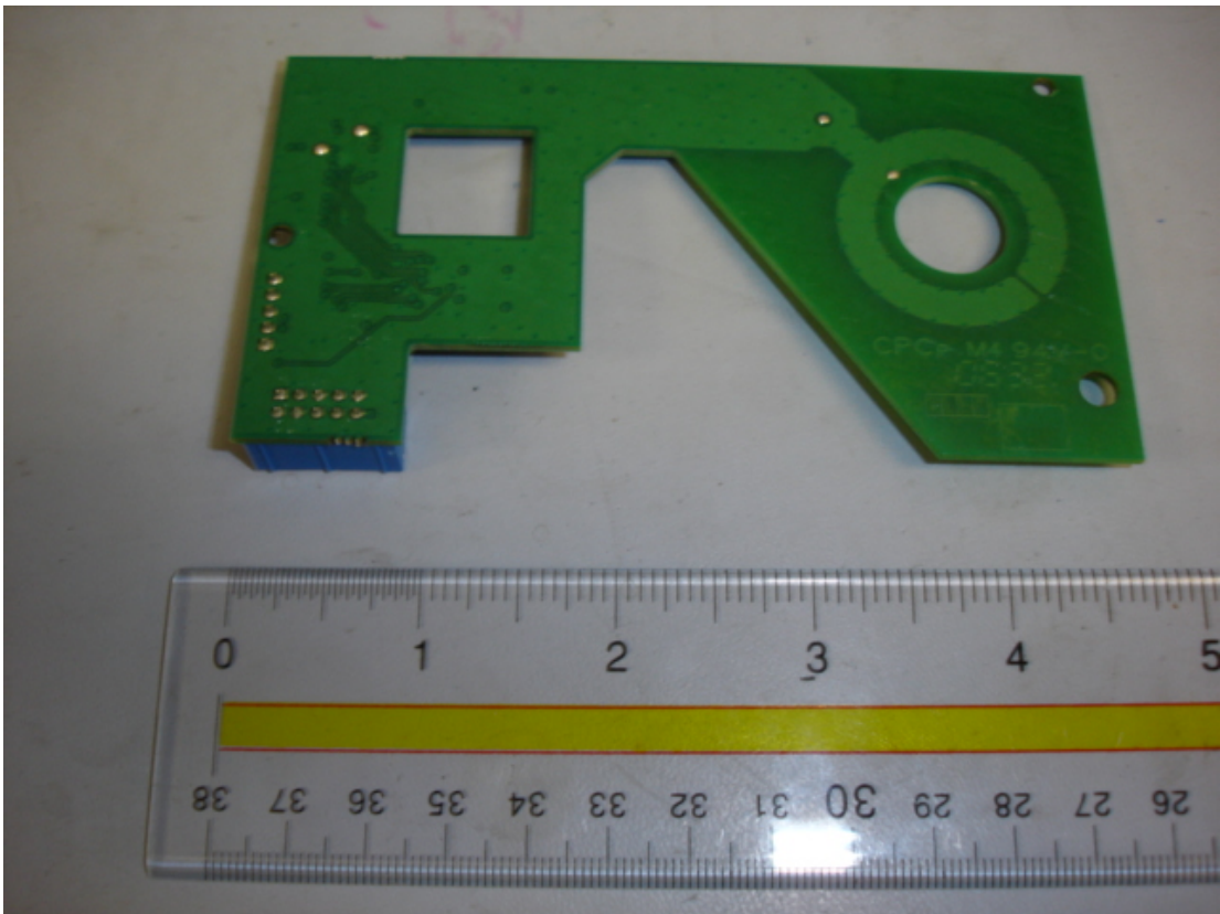
RFID Radio board Bottom View
