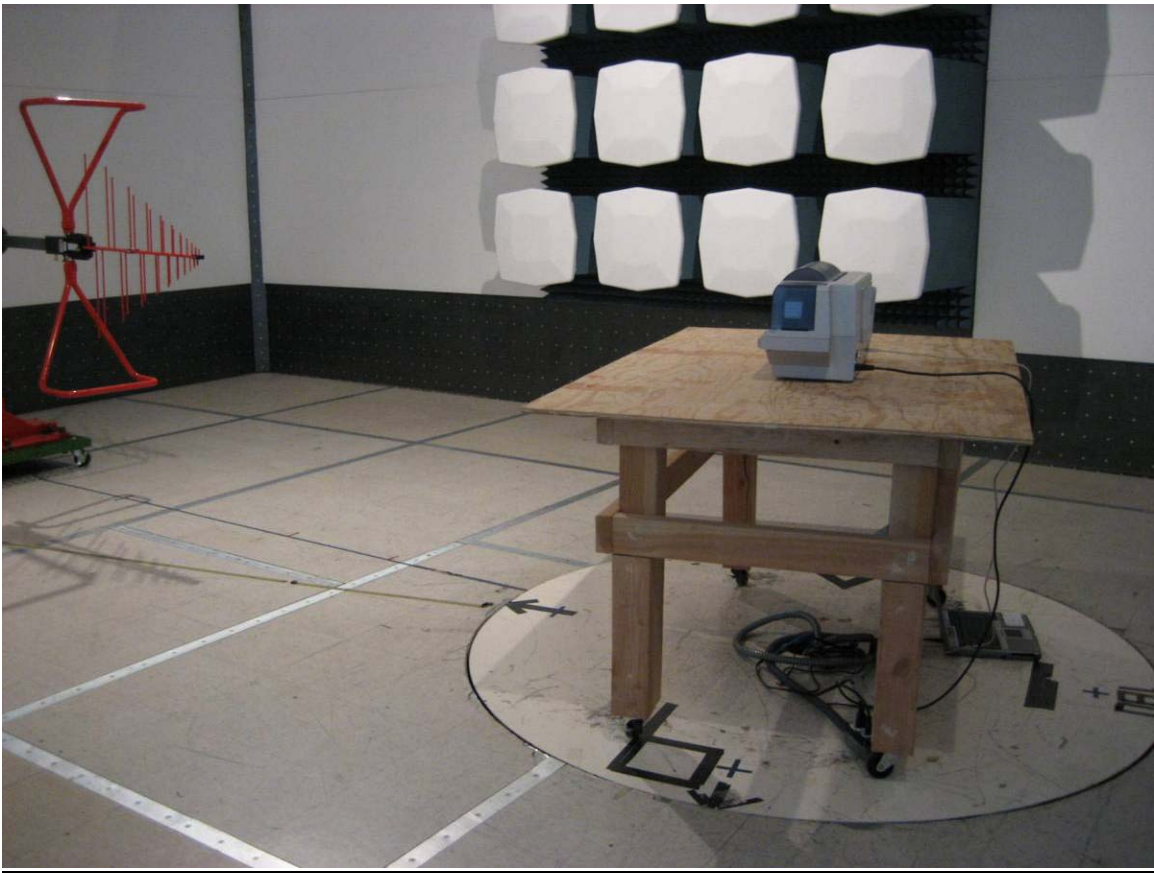
Radiated Emission Test Setup View (30MHz~1000MHz)
