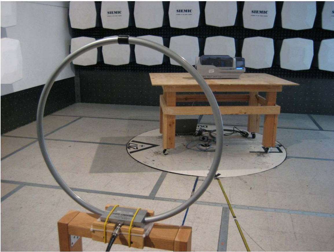
Radiated Emission Test Setup View (<30MHz)
