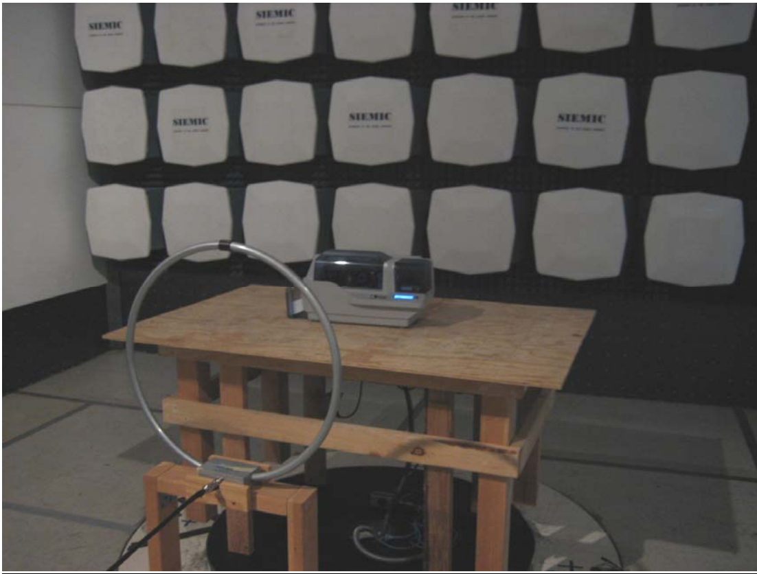
Radiated Emission Test Front View (<30MHz)
