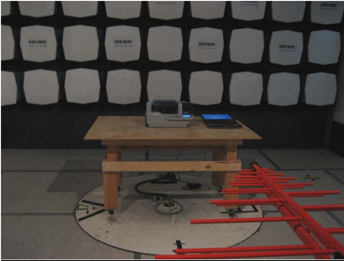
Radiated Emission Test Setup Front View (<1000MHz)
