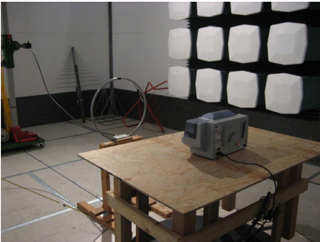
Radiated Emission Test Rear View (<30MHz)
