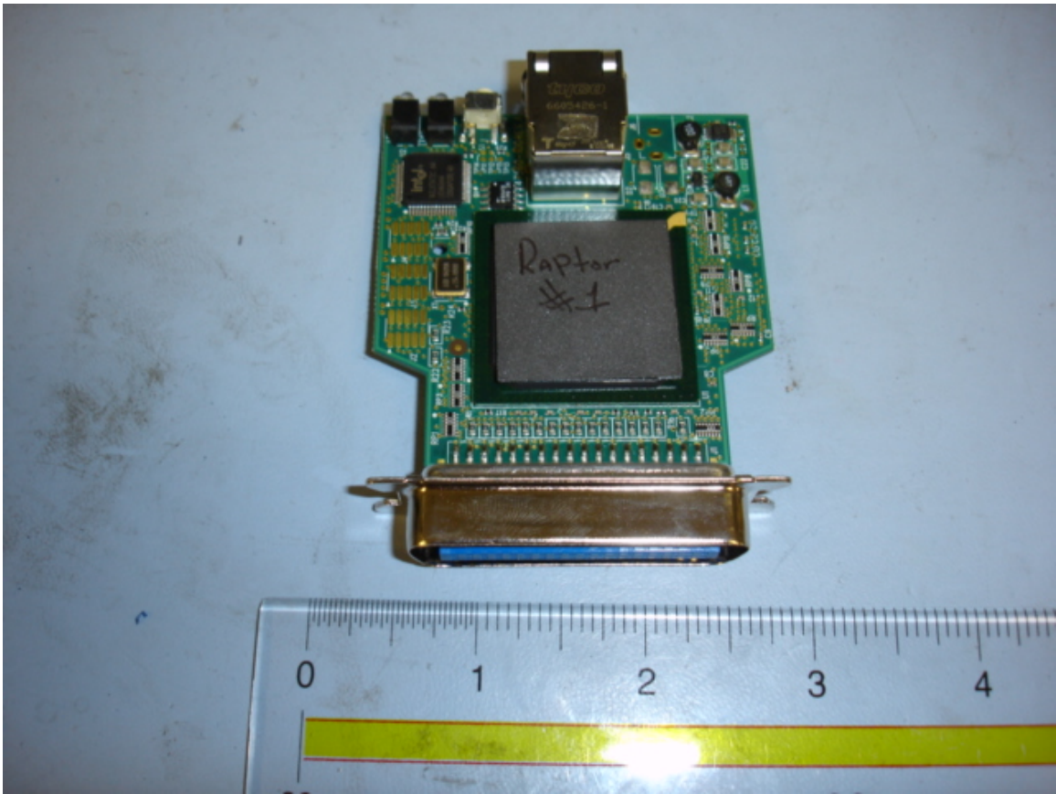
Ethernet Board Top View
