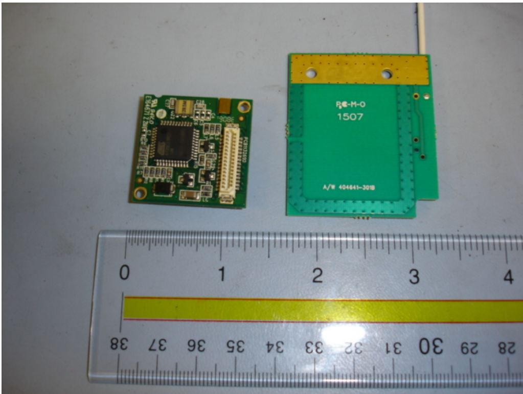
Mifare radio and antenna Bottom View
