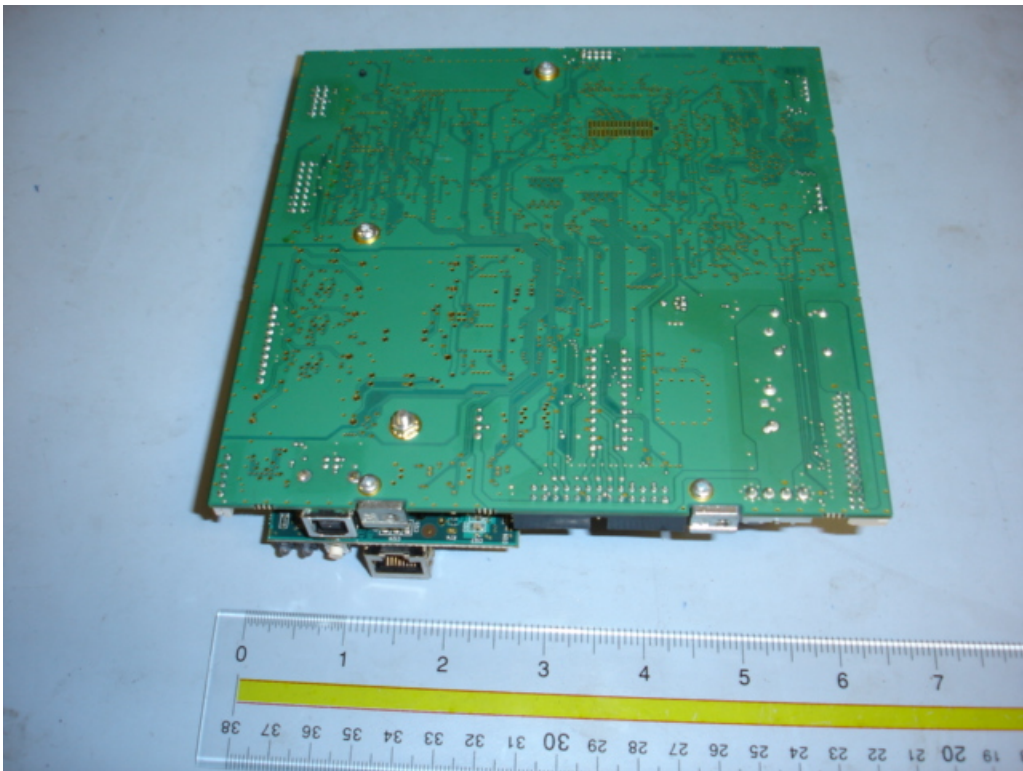
Main Board 1 with USB Bottom View
