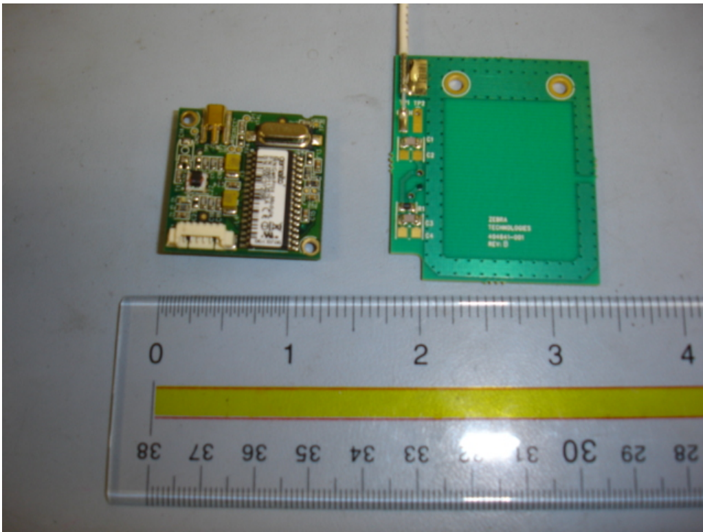
Mifare radio and antenna Top View
