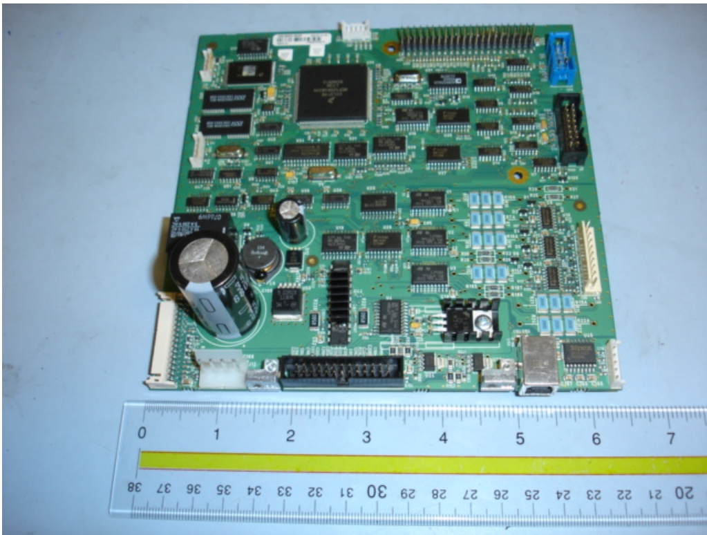
Main Board 1 with USB Top View
