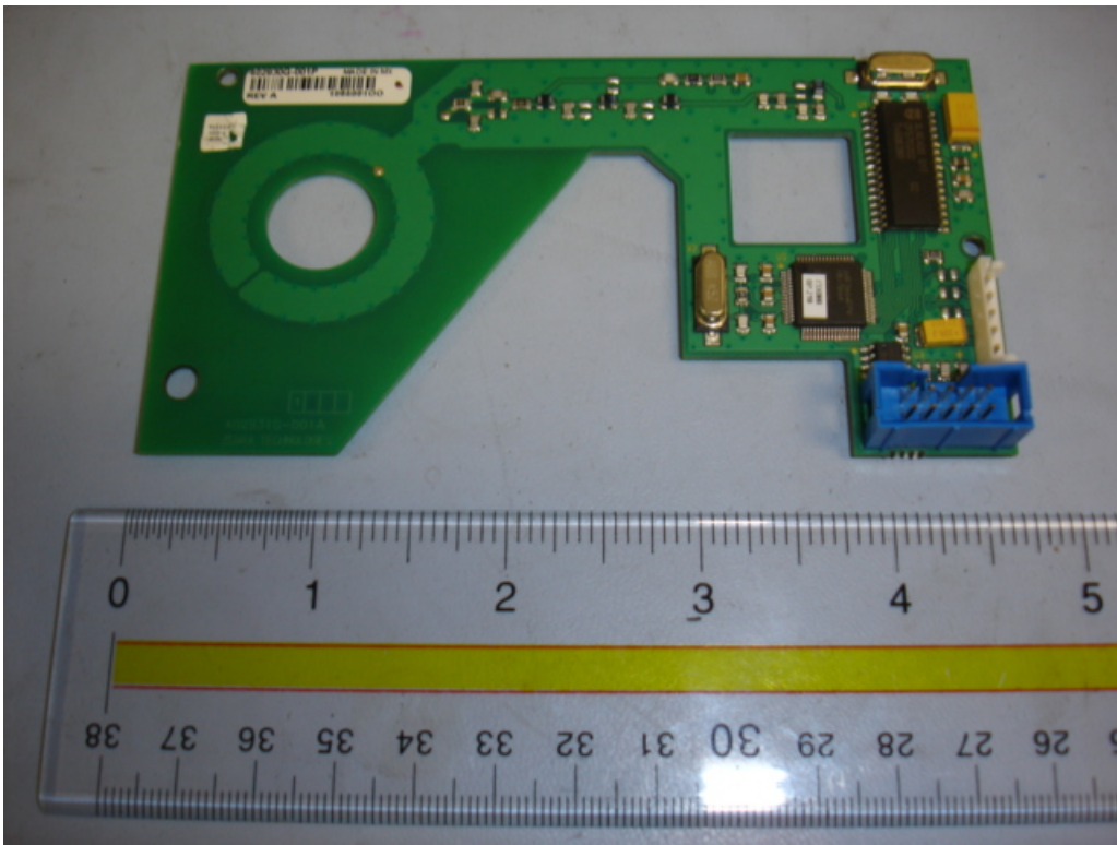
RFID Radio board Top View
