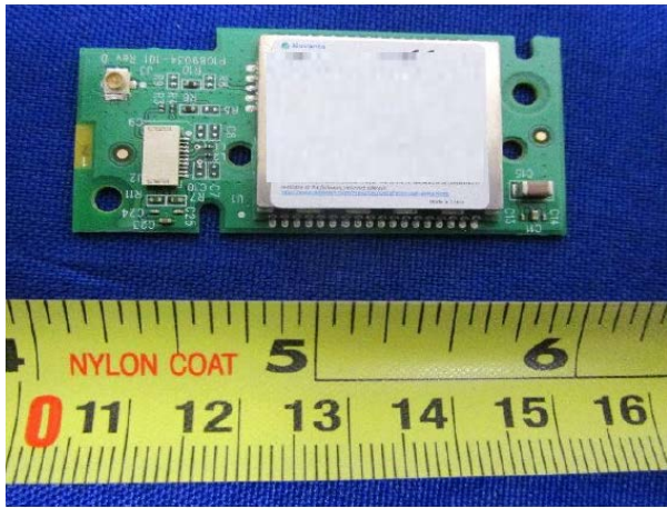
RFID Radio Module - Top View
