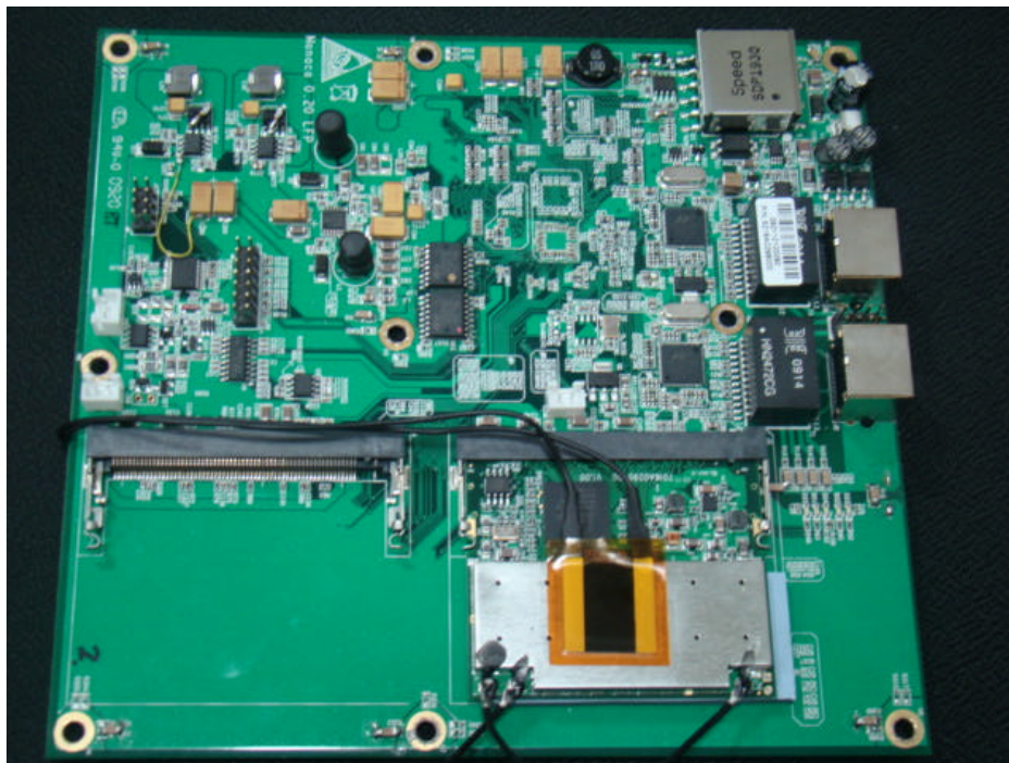
PCB with RF Module without - Top View
