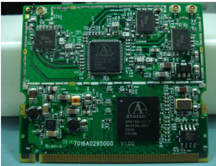
RF Module without shield - Top View
