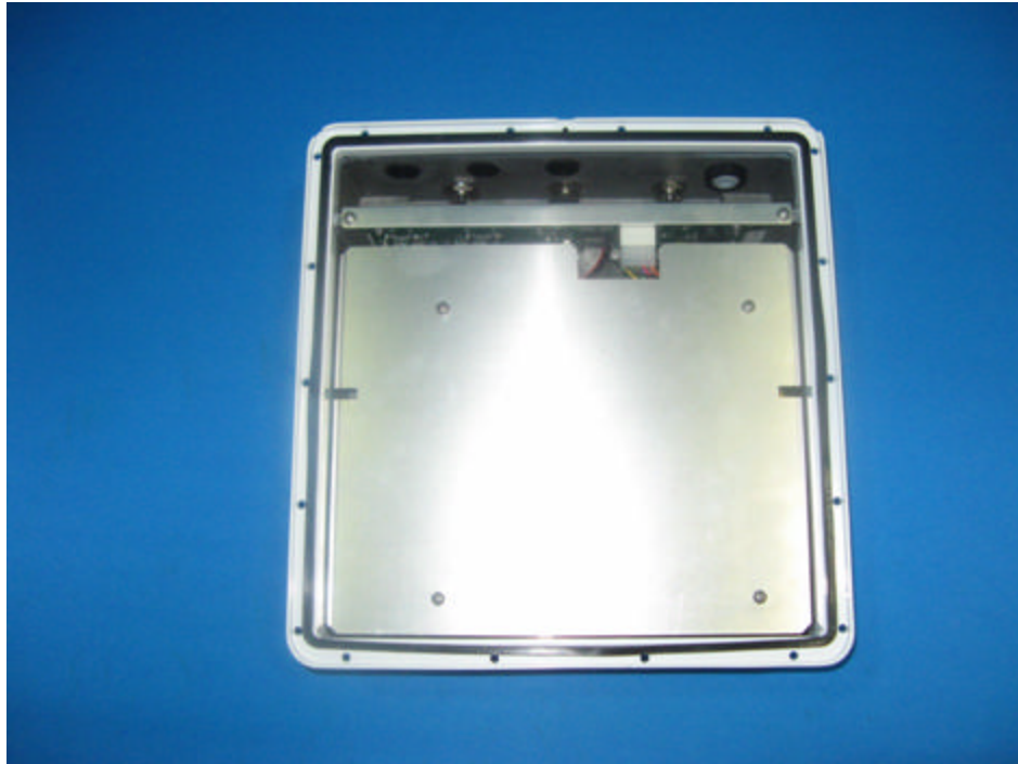
Bottom Cover – Internal View PCB with cover
