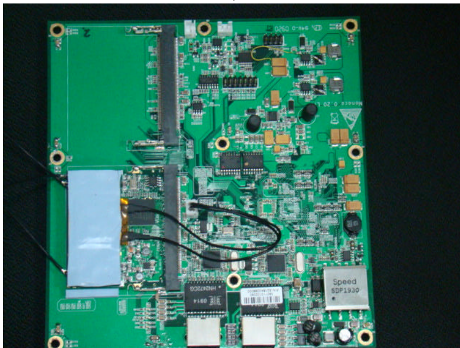
PCB with RF Module with Shield – Top View
