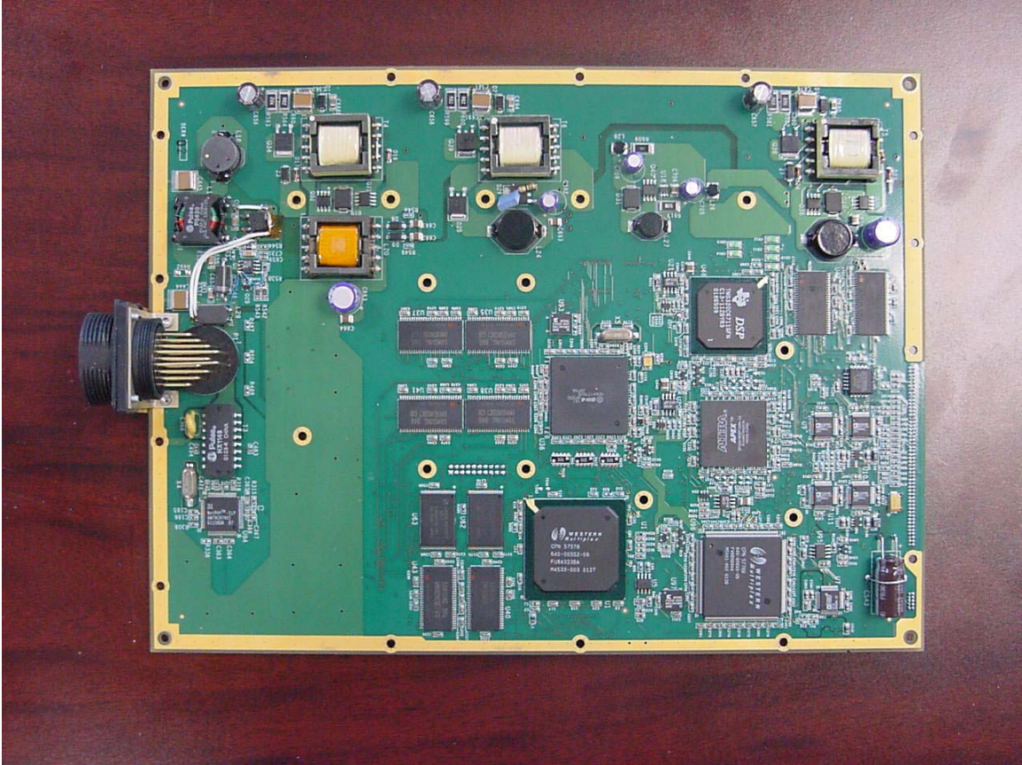
Digital board (bottom view)
