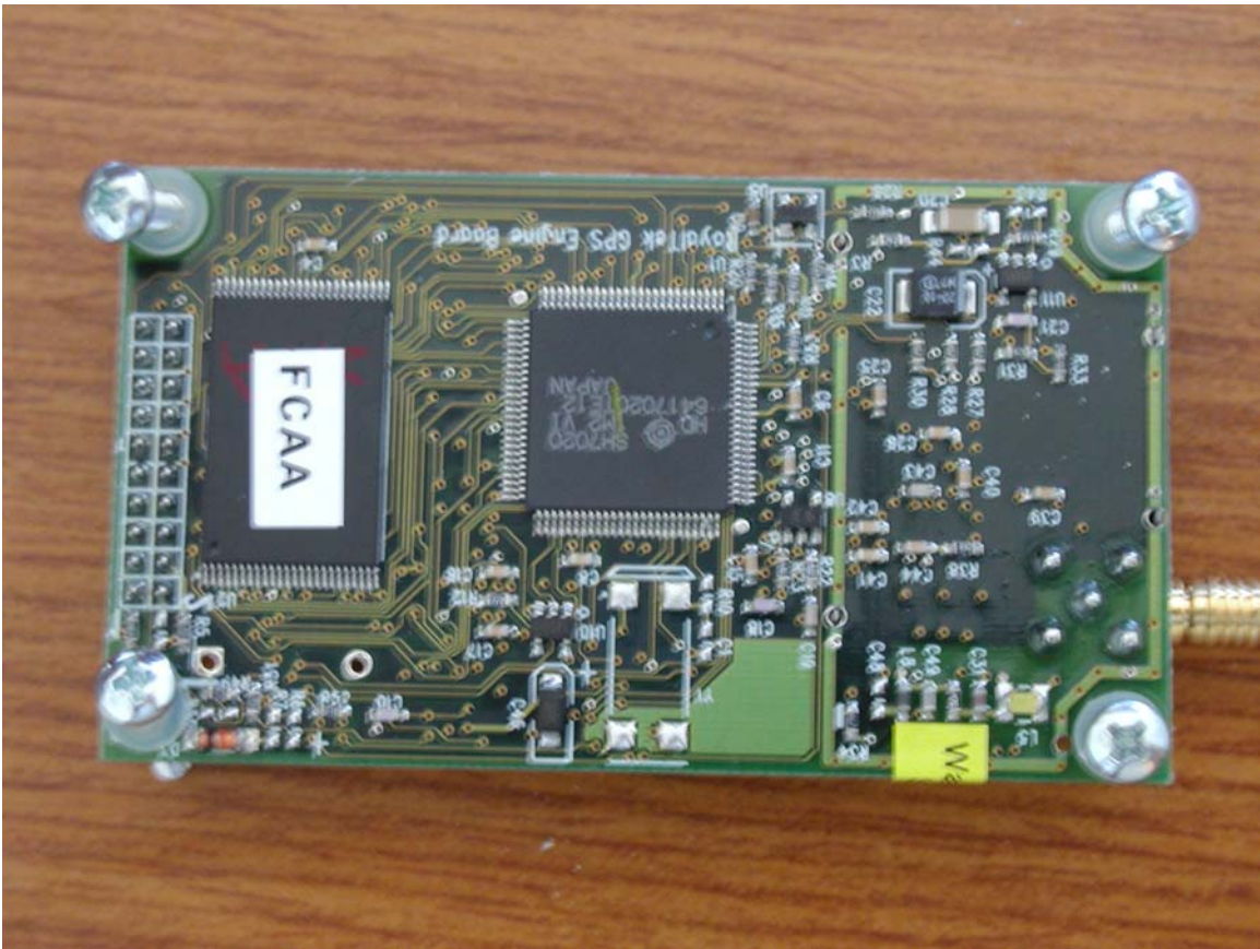
GPS receiver (top view)
