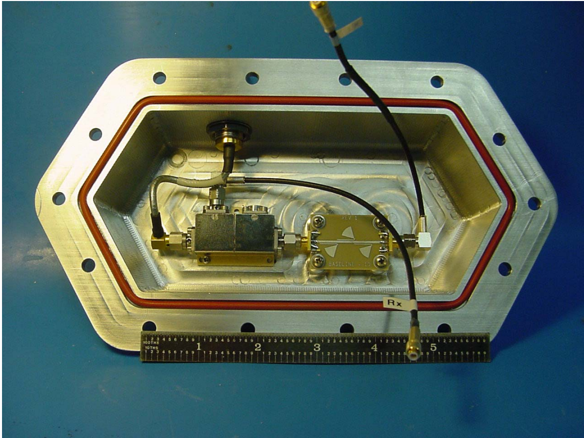
Connectorized BSU
