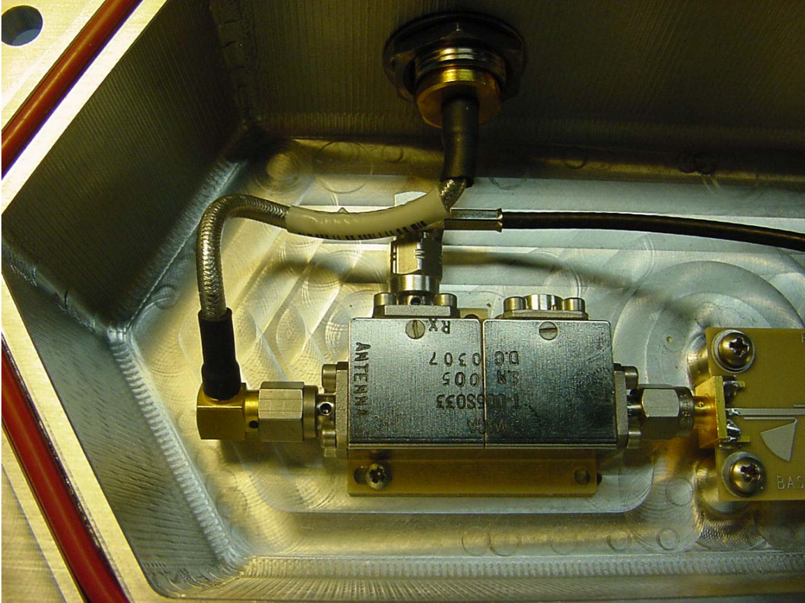
Connectorized BSU
