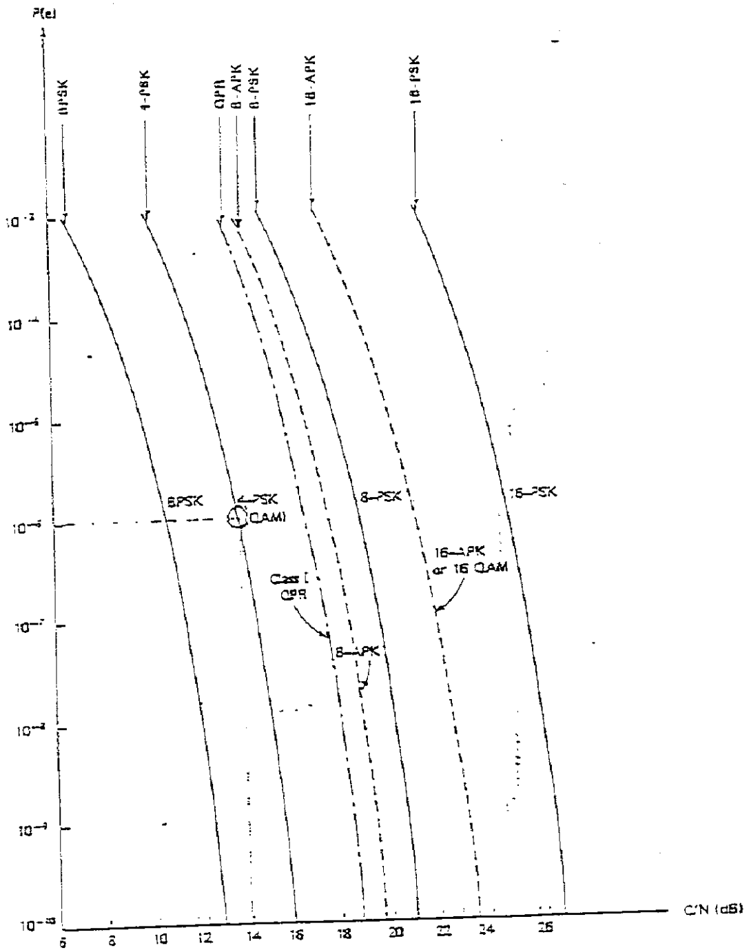
Fig. 1.11 P(e) performance of M -ary PSK, QAM, QPSK, and M -ary APK coherent systems. The rms C/N is specified in the double-sided Nyquist bandwidth.
