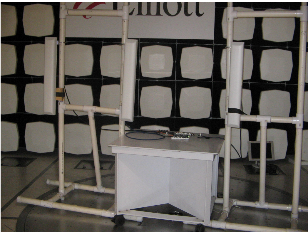
General configuration for Panel (top) and Sector (bottom) antennas. All antennas were aligned and pointing in the same direction.
