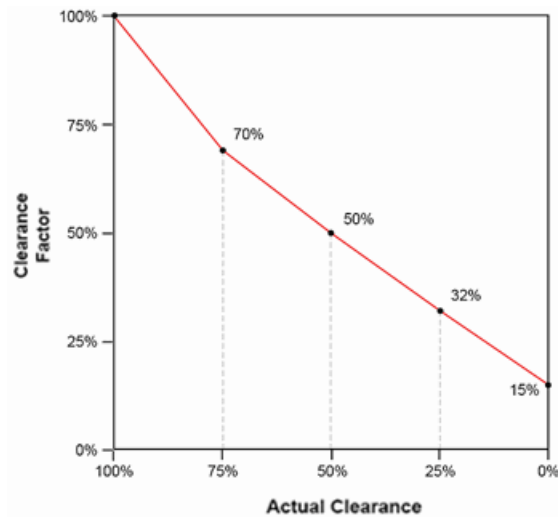
Figure 9-3 Clearance Factor
