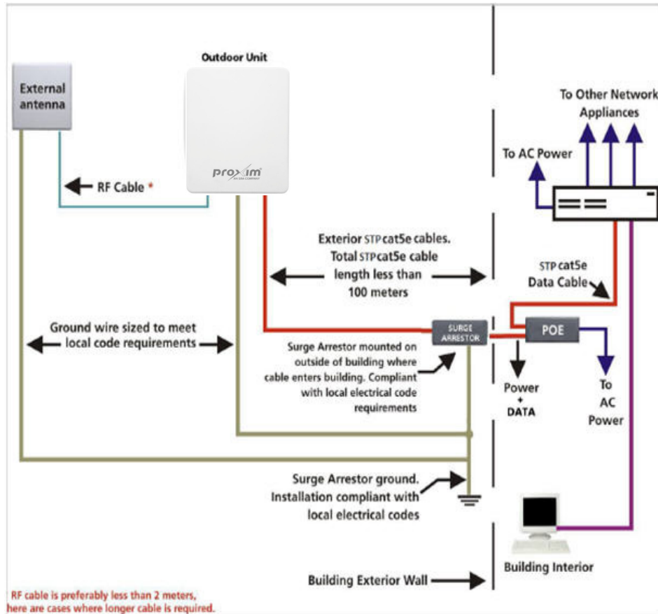
Figure 8-7 Cable Setup
