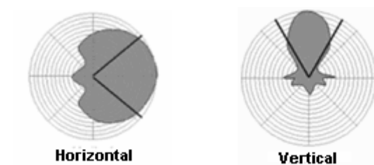
Figure 7-2 Sector Antenna Coverage
