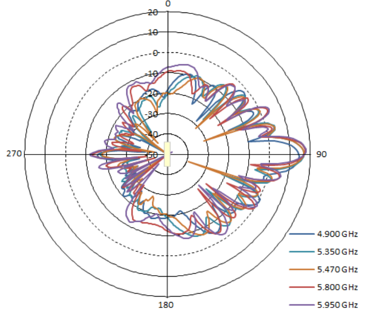
H-pol Elevation
