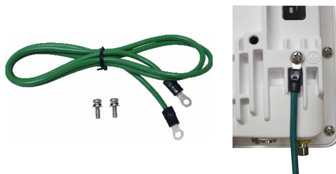
Figure 4-6 Ground the Device
