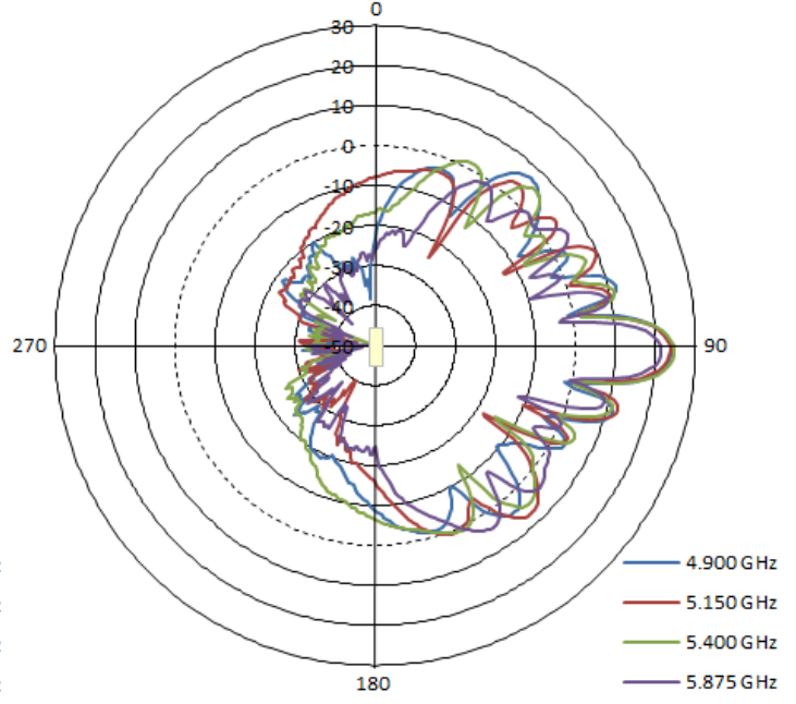
H-pol Elevation
