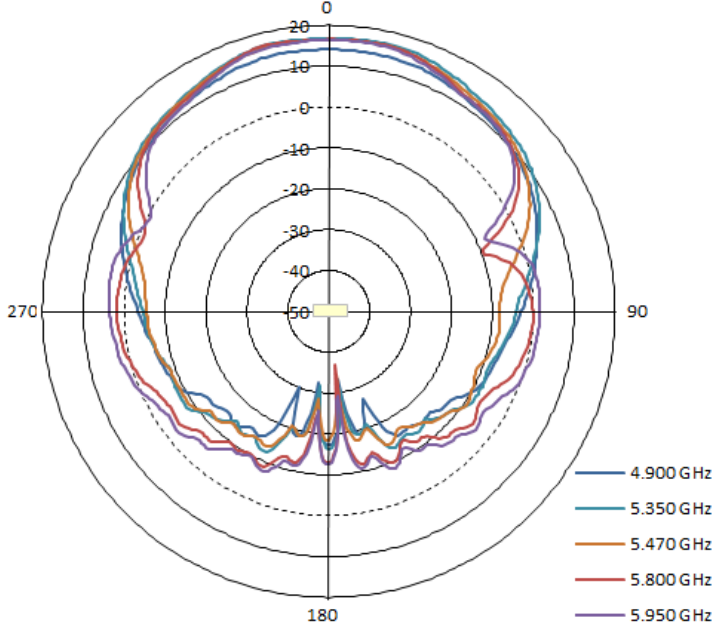
H-pol Azimuth
