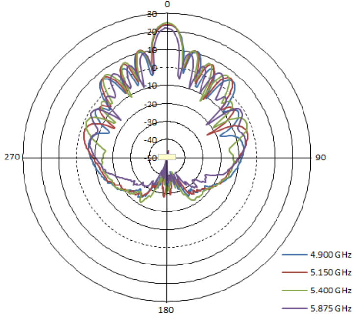
H-pol Azimuth
