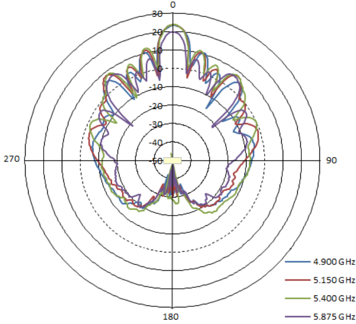
V-pol Azimuth
