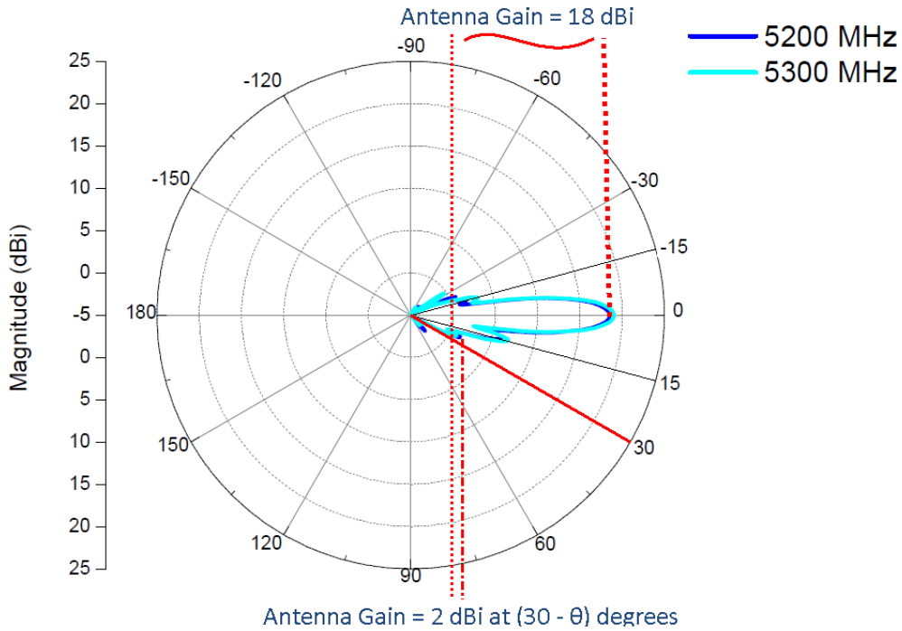
Figure 8-4 Antenna gain at (30 - 0) = 30^\circ
