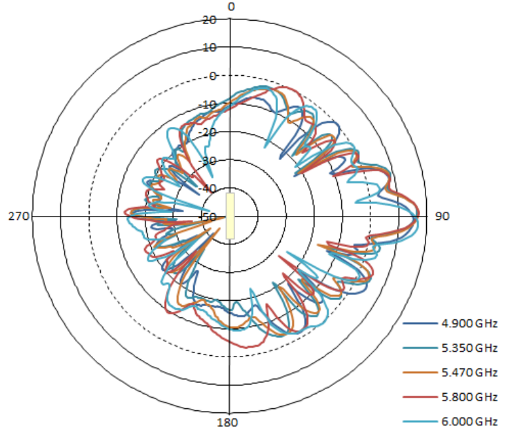
H-pol Elevation
