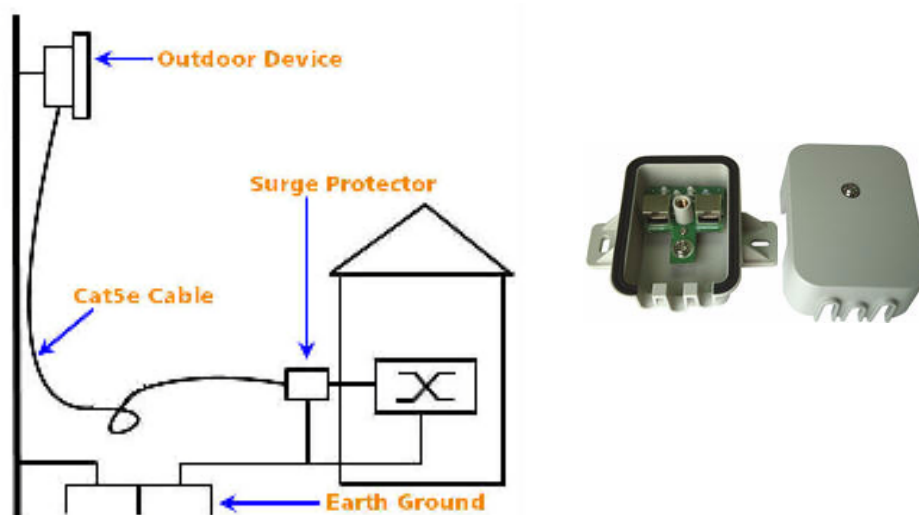
Figure 4-5 Surge Protector
