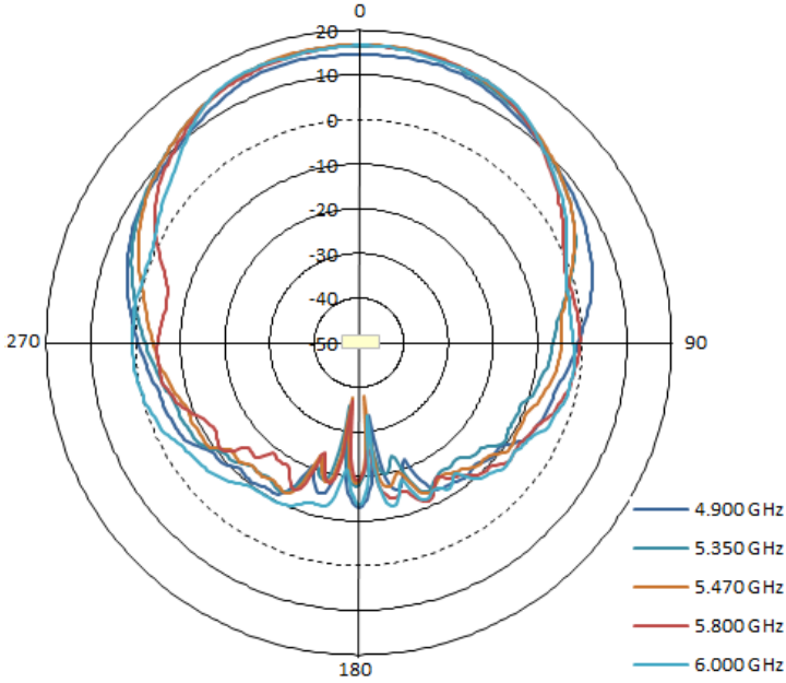
H-pol Azimuth
