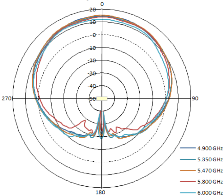
V-pol Azimuth
