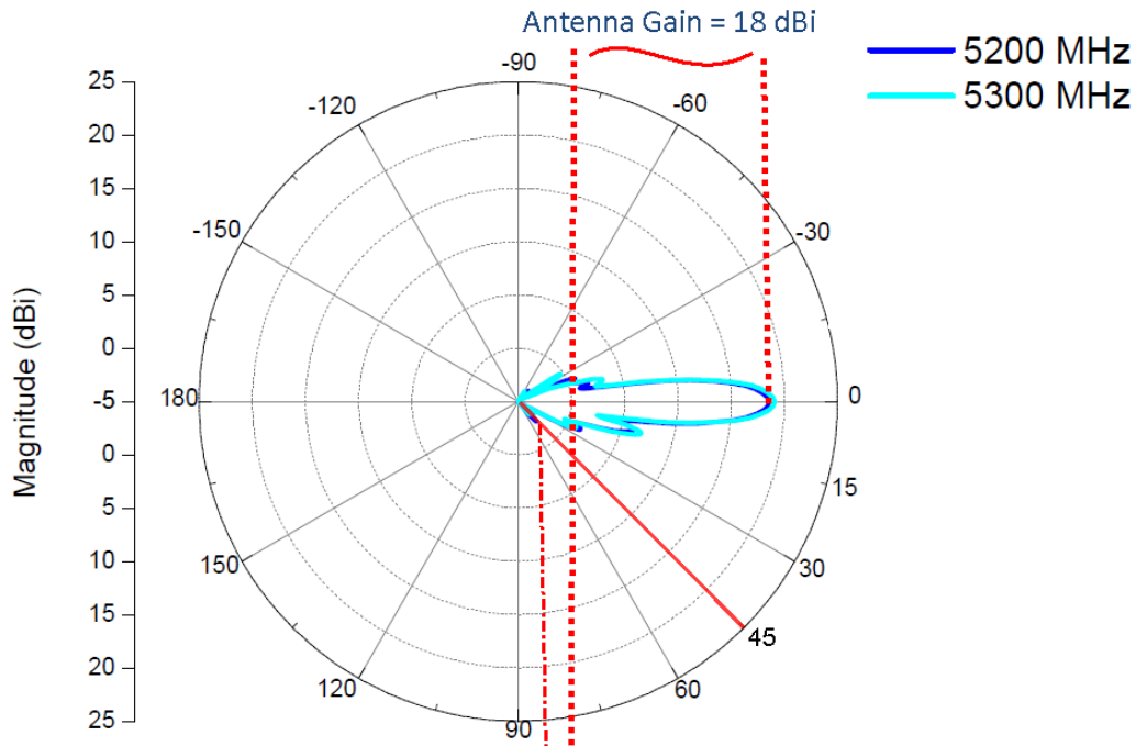
Figure 8-6 Antenna gain at (30 - \theta) = 45^\circ
