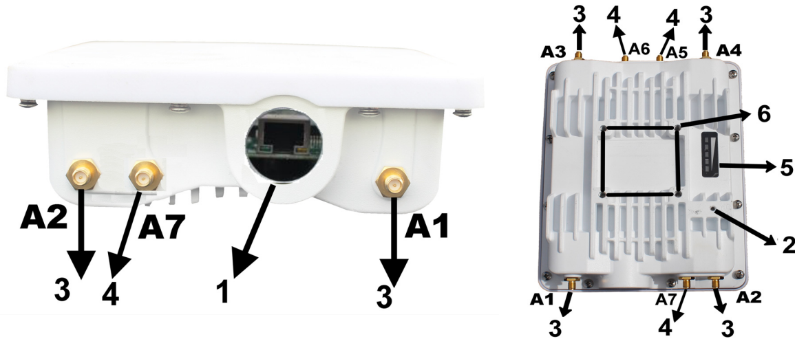
Figure 3-1 AP9200R
