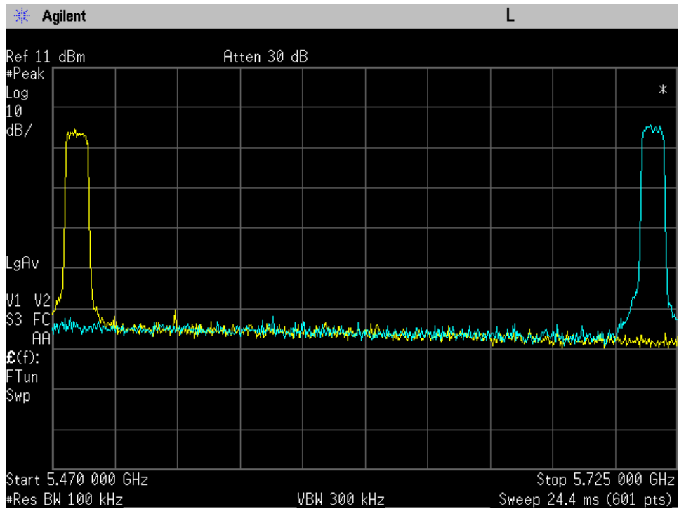
UNII-2C 25deg C
