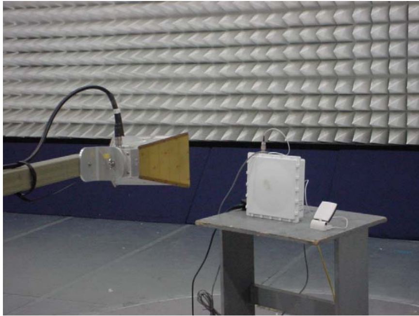
Patch antenna
