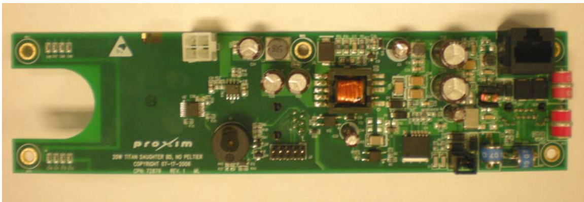
Power Supply Board - Component Side
