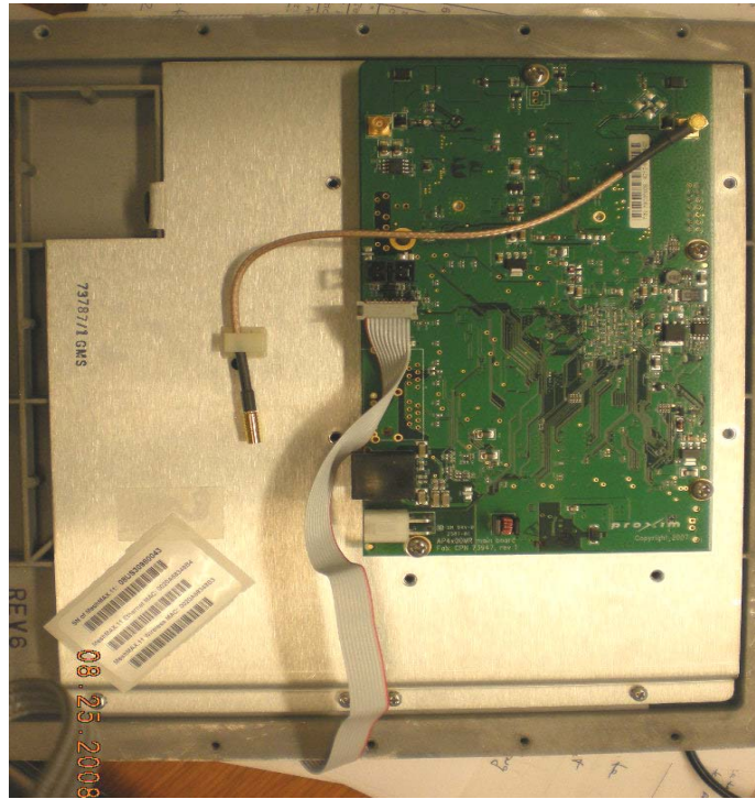
Radio Board – Cover mount
