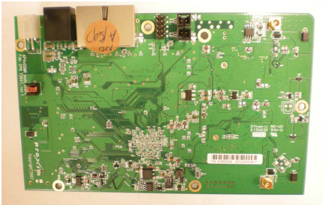
Radio Board Front Side
