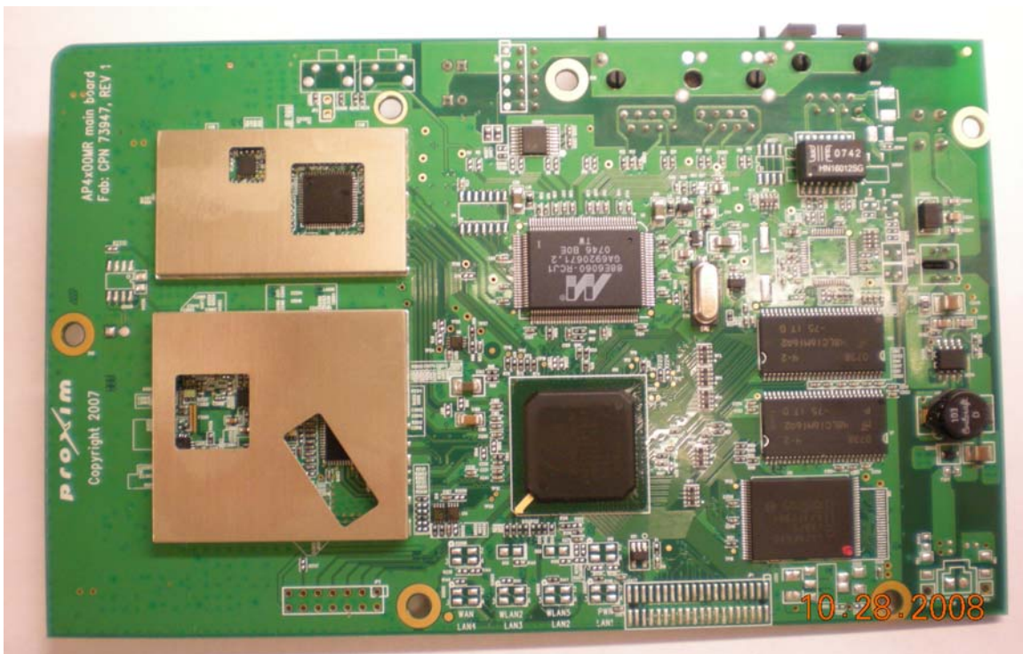
Radio Board - Component Side
