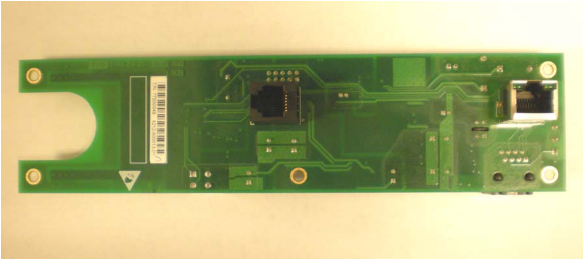
Power Supply - Connectors Side
