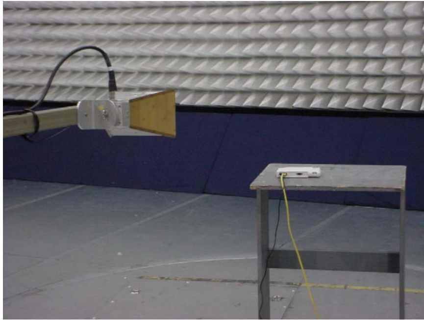
Internal antenna
