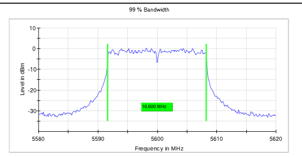
Channel Frequency:5600MHz
