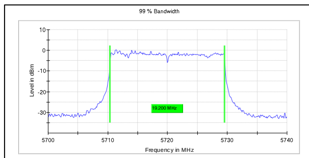
Channel Frequency:5720MHz
