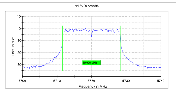
Channel Frequency:5720MHz
