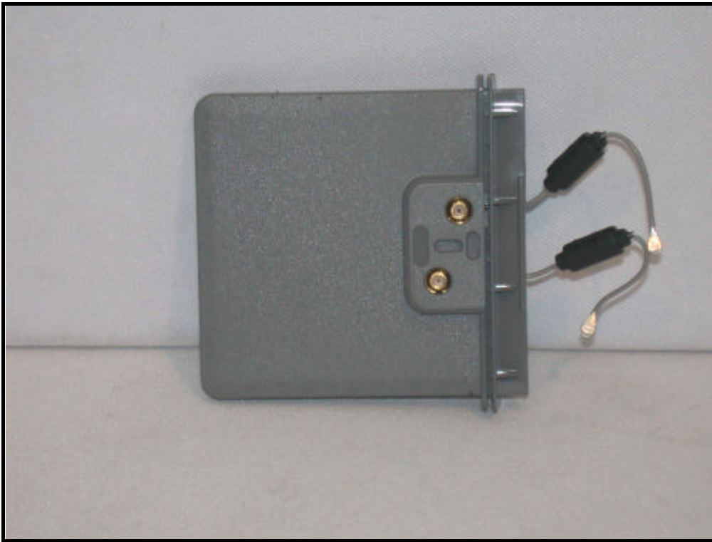
Antenna 1
