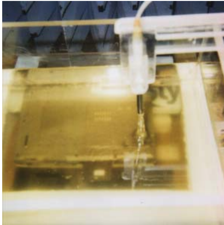
Fig. 5. Photograph of the Proxim Europe B.V. Model 8460-05 Cardbus Card inserted into a laptop computer with its bottom pressed against the bottom of the planar tissue-simulant phantom to simulate "above-lap" placement of the wireless PC. A Styrofoam block is used under the base to prevent bending of the 2 mm thin base of the phantom.
