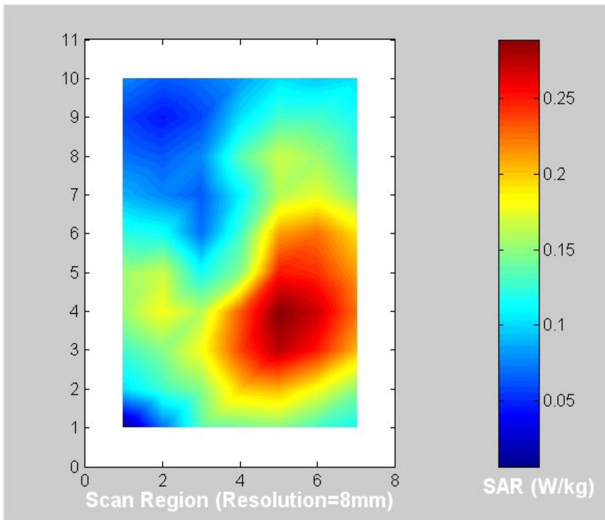
(b) 5.785 GHz base mode (see Table 8 for the peak 1-g SAR).
