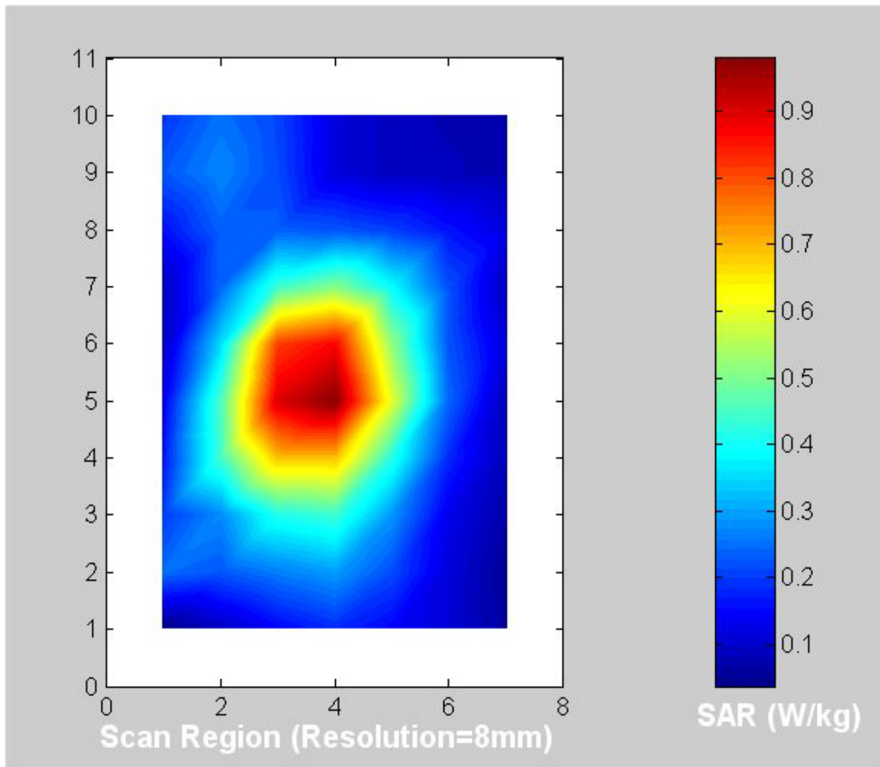
(a) 5.26 GHz base mode (see Table 3 for the peak 1-g SAR).
