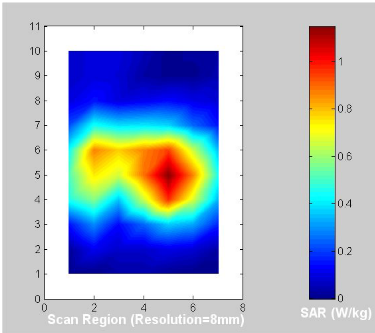
(b) 5.785 GHz base mode (see Table 4 for the peak 1-g SAR).
