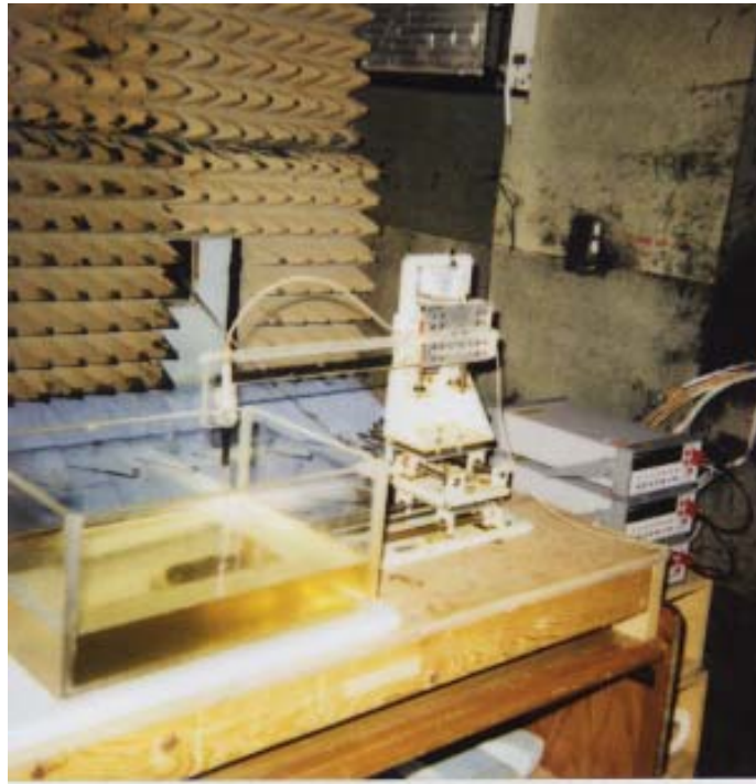
Fig. 3. Photograph of the three-dimensional stepper-motor-controlled SAR measurement system using a planar phantom (see Fig. 5 for a detailed examination of the placement of Proxim Europe B.V. Model 8460-05 Cardbus Card relative to this phantom).
