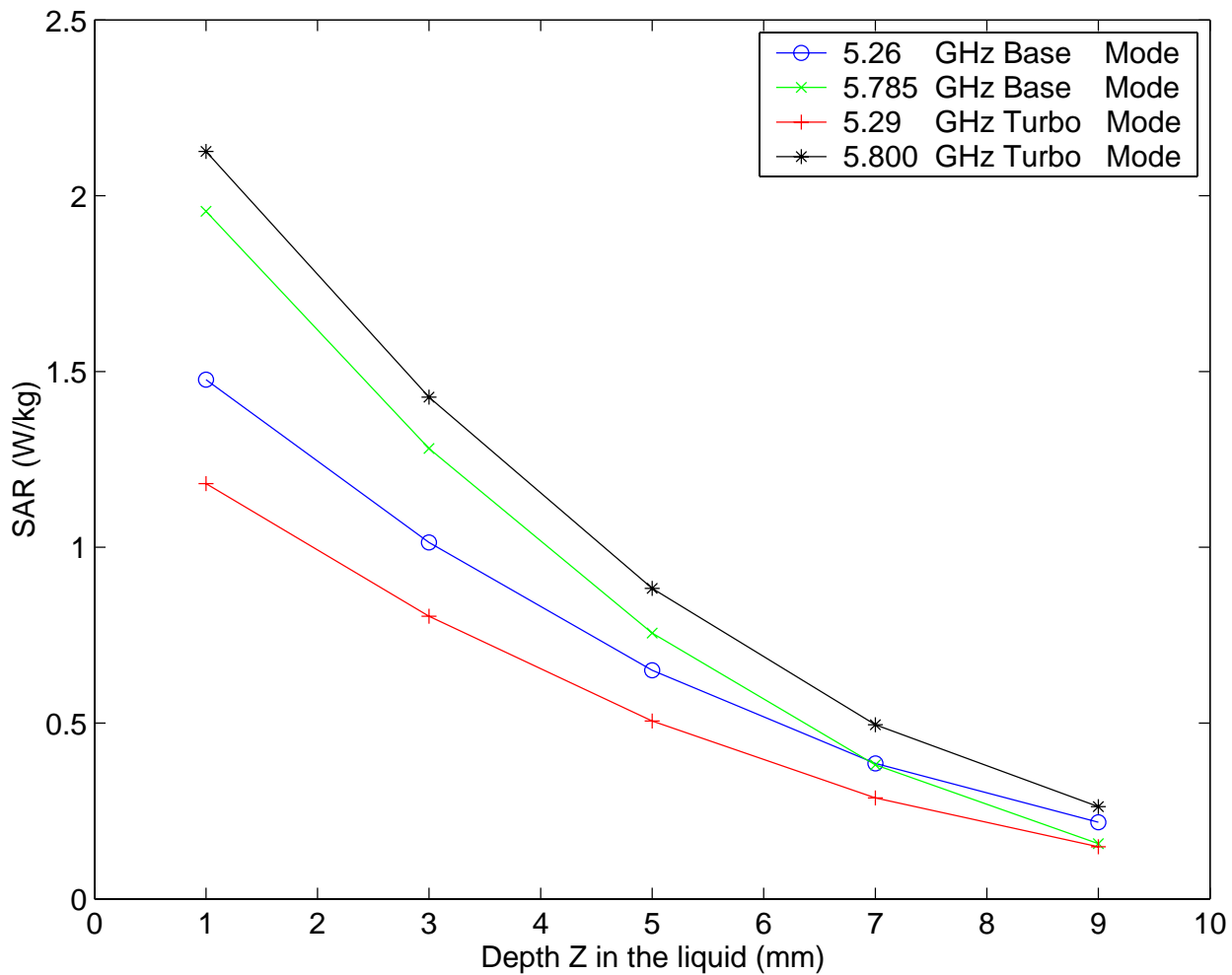
Fig. 16. Plot of the SAR variations as a function of depth Z in the liquid for locations of highest SAR (from Tables 3-6 -- Above-lap position) for the Proxim Europe B.V. Model 8460-05 Cardbus Card.
